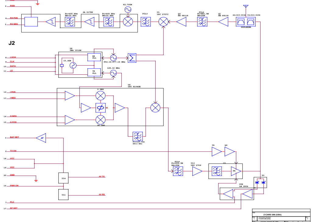
Figure 4-2 VG300 Radio Block Diagram
