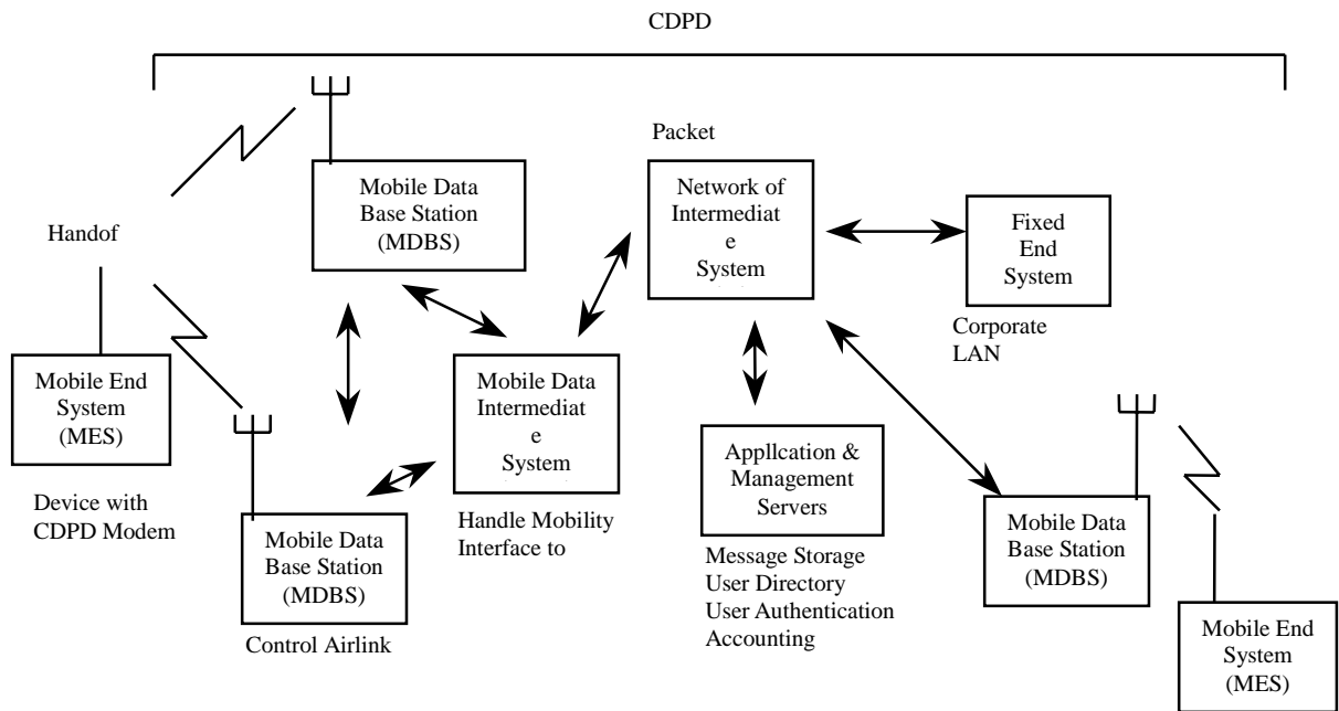
Figure 4-1 CDPD Network
