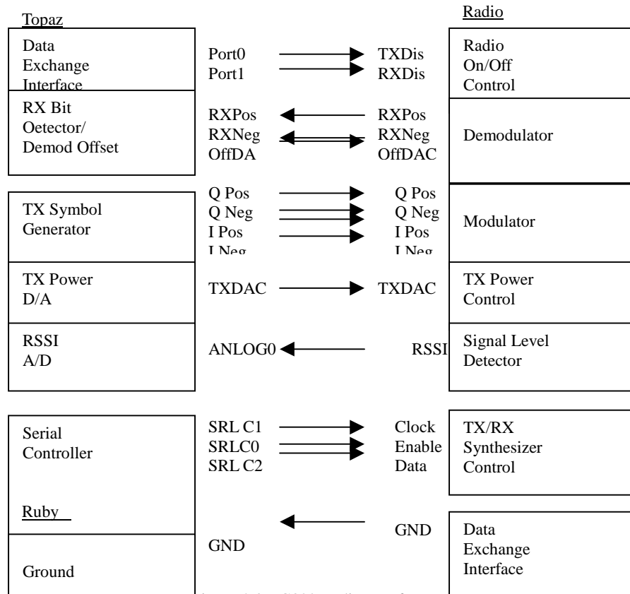
Figure 4-3 VG300 Radio Interface
