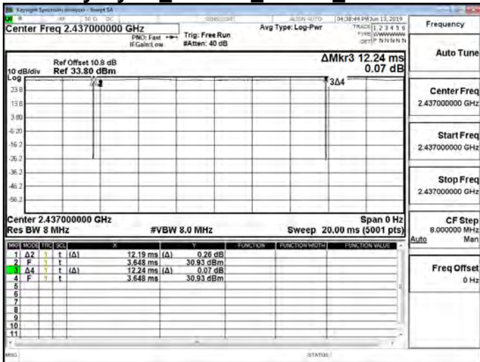
Duty Cycle_802.11g_20MHz_2437MHz
