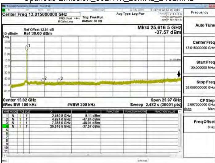
Spurious Emission_802.11n_20MHz_2462MHz
