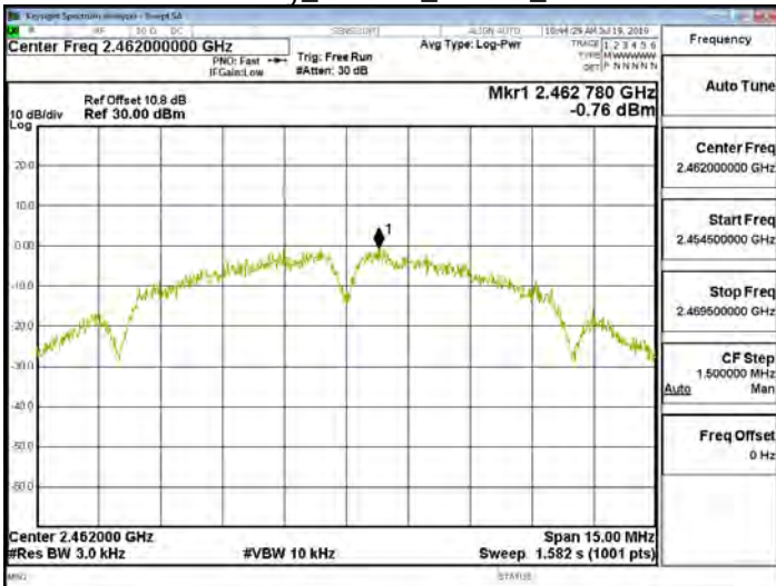
Power Density_802.11b_20MHz_2462MHz
