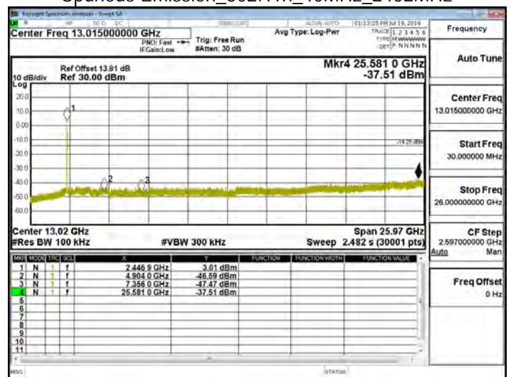
Spurious Emission_802.11n_40MHz_2452MHz
