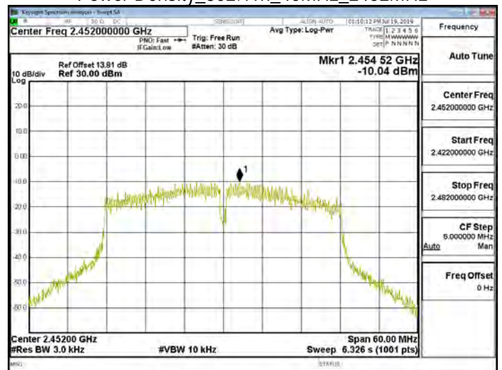
Power Density_802.11n_40MHz_2452MHz
