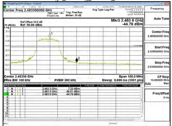
Band Edge_802.11g_20MHz_2462MHz
