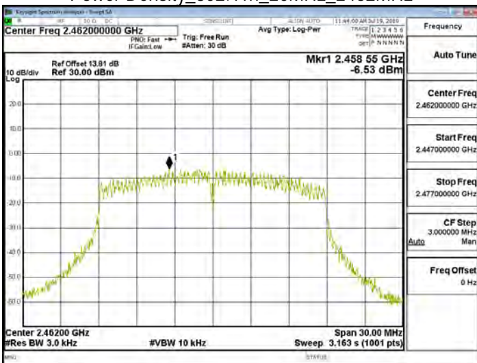
Power Density_802.11n_20MHz_2462MHz
