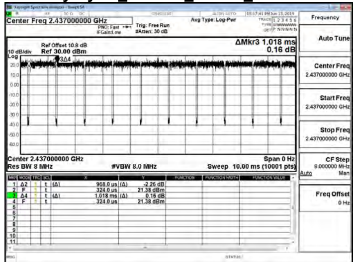
Duty Cycle_802.11n_40MHz_2437MHz
