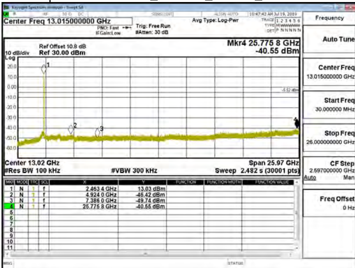
Spurious Emission_802.11b_20MHz_2462MHz
