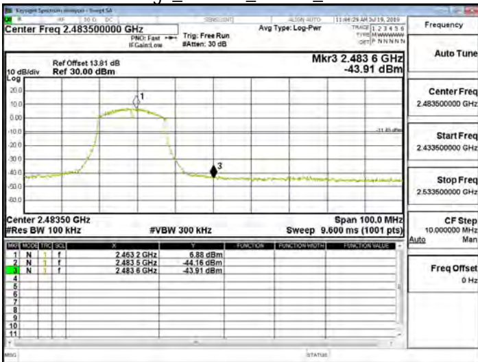
Band Edge_802.11n_20MHz_2462MHz
