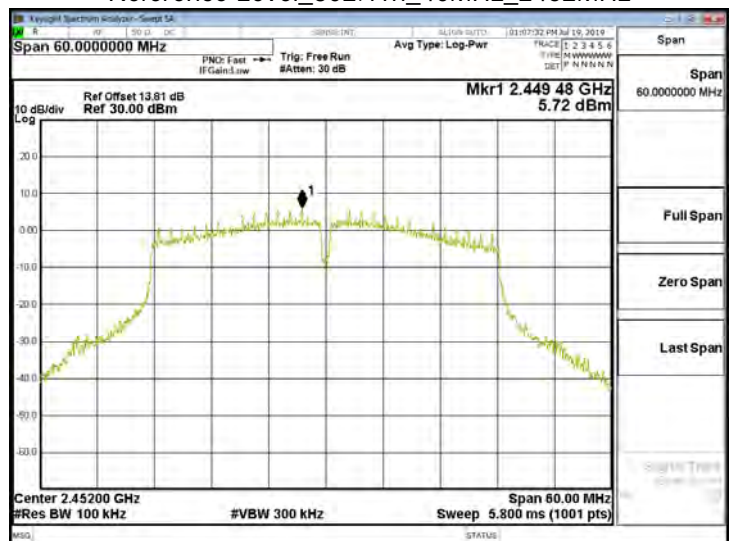
Reference Level_802.11n_40MHz_2452MHz
