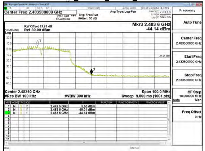
Band Edge_802.11n_40MHz_2452MHz
