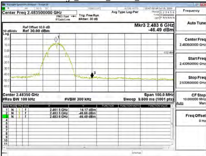
Band Edge_802.11b_20MHz_2462MHz
