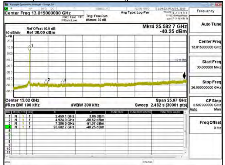
Spurious Emission_802.11g_20MHz_2462MHz
