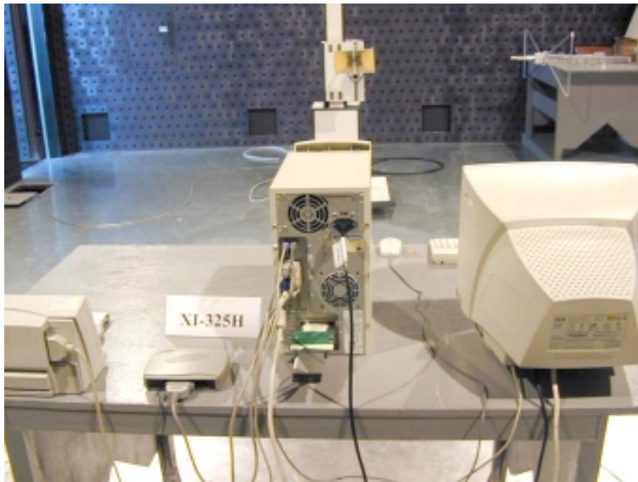
Photo 3: Spurious test set-up photo
