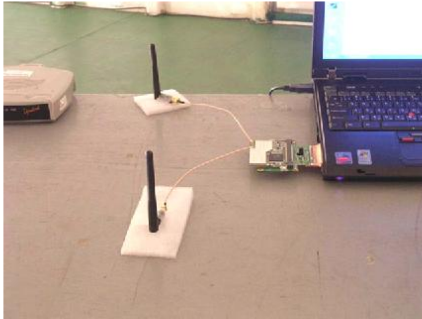
Photo 3: Radiated Emission Test Set-up
