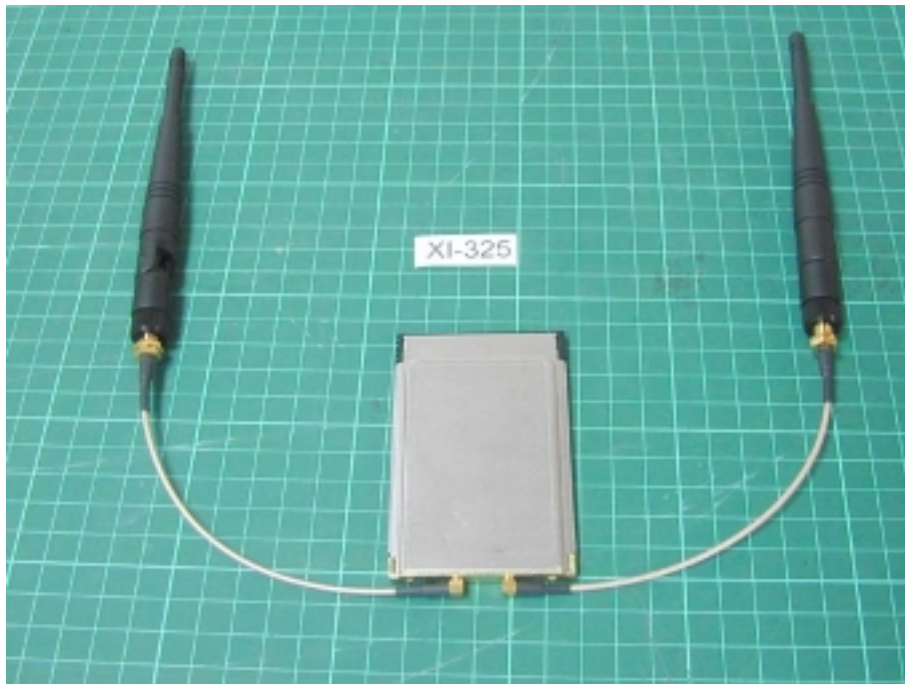
Photo 3: EUT with antenna (antenna gain is 2dBi)
