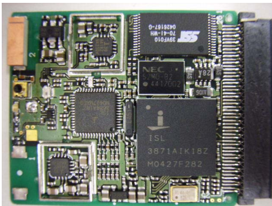
RF Module-Top (Cover off2)
