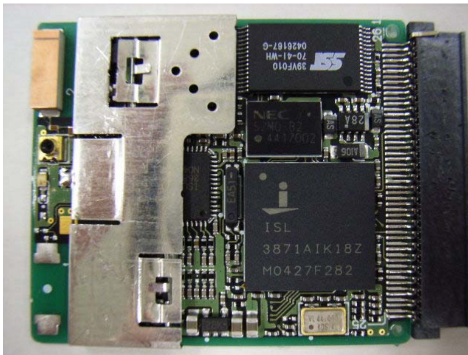
RF Module-Top (Cover off 1)
