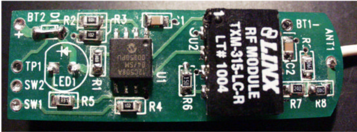
WRC TRANSMITTER PCA COMPONENT SIDE
