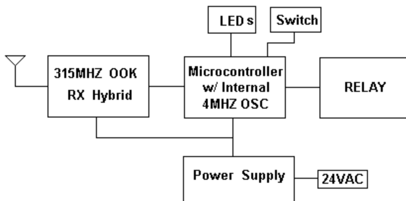
WRC Receiver Block Diagram
