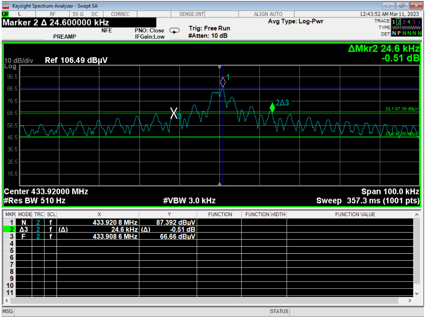
-20 dB Bandwidth Plot – U3 Version
