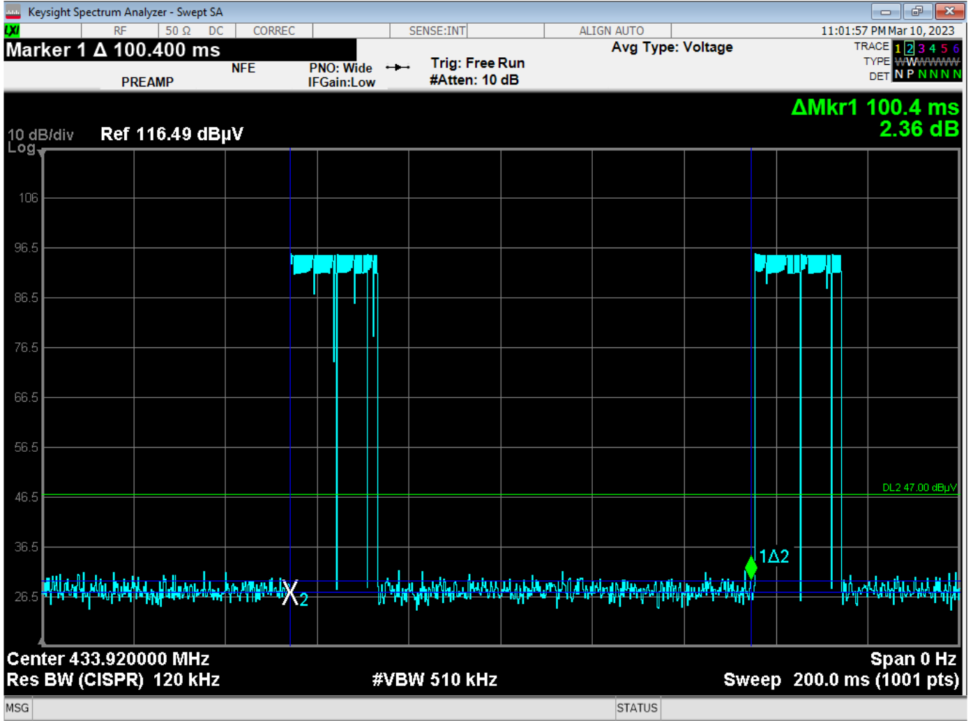
The pulse train only appears once every 100 ms – U2 Version
