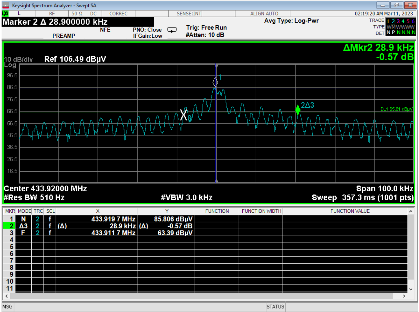
-20 dB Bandwidth Plot – U2 Version
