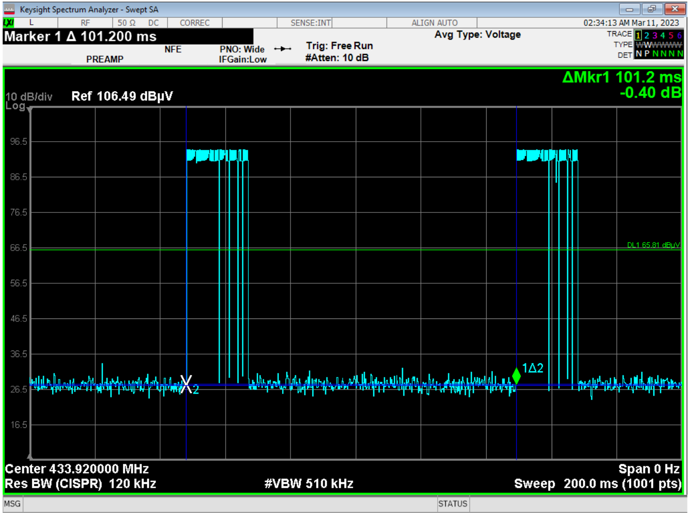
The pulse train only appears once every 100 ms – U3 Version
