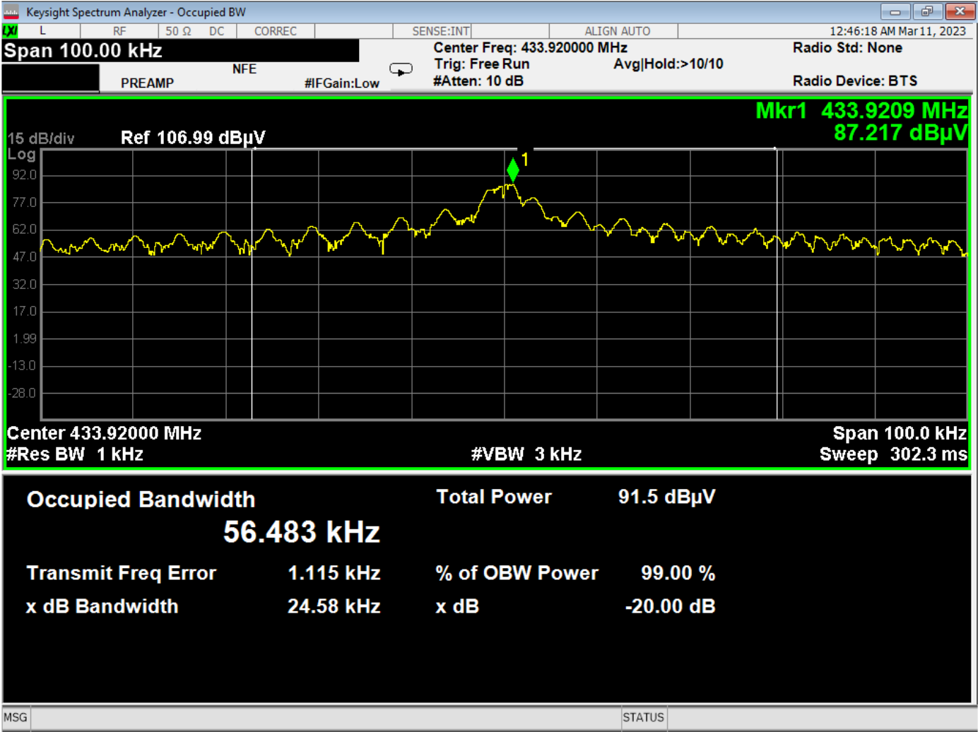
99 Percent Bandwidth Plot – U3 Version
