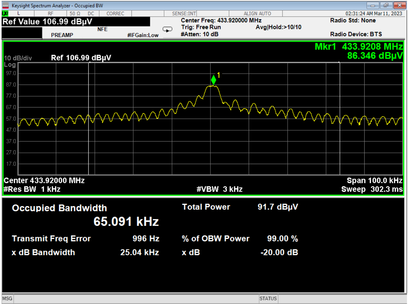
99 Percent Bandwidth Plot – U2 Version
