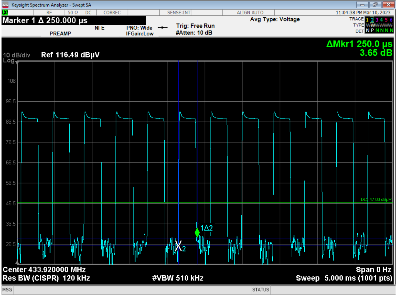
Time of Small Pulse = 250 us – U2 Version
