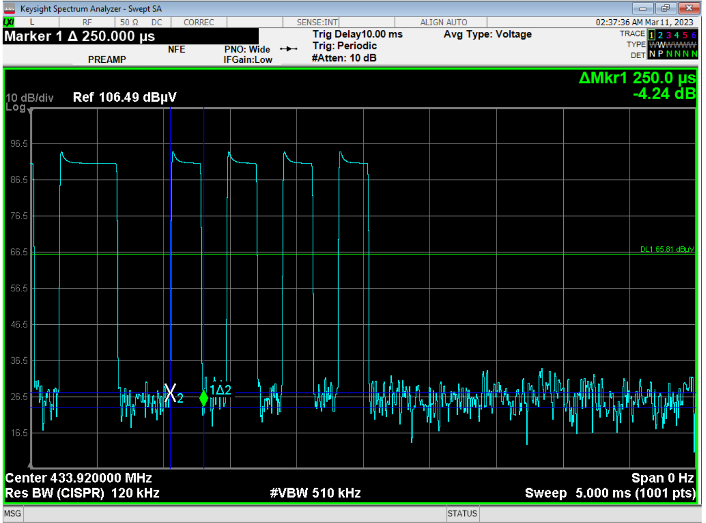
Time of Small Pulse = 250 us – U3 Version
