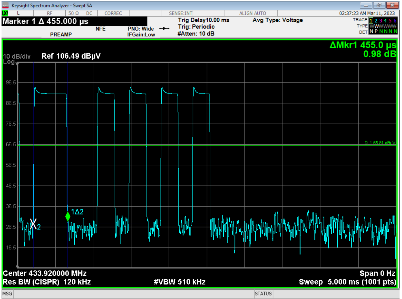
Time of Large Pulse = 455 us – U3 Version
