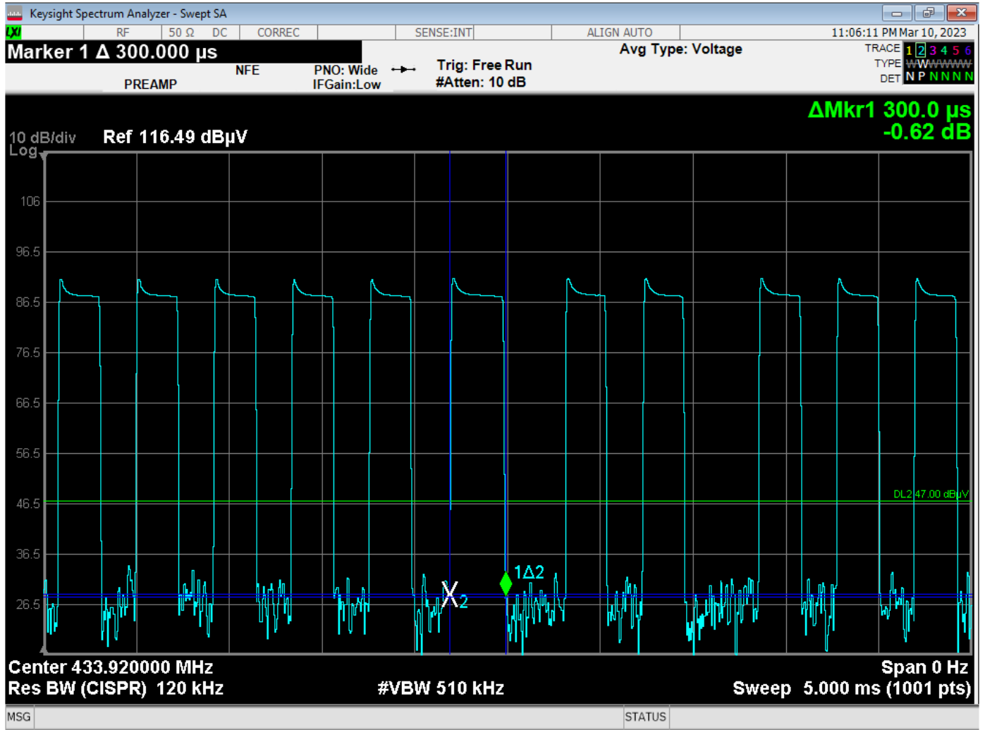
Time of Large Pulse = 300 us – U2 Version
