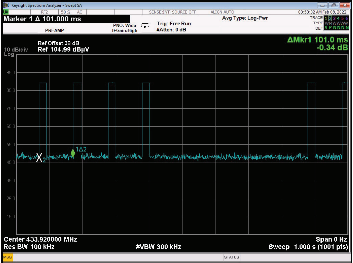
The pulse train only appears once every 100 ms
