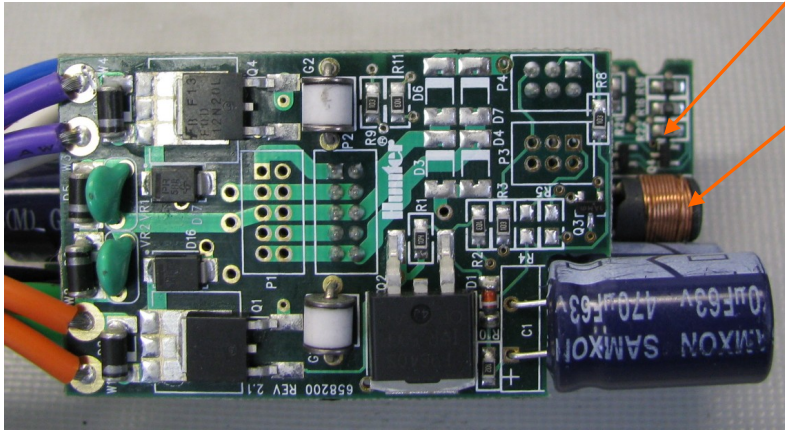
Top View, Full Assembly
