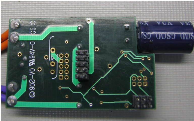
Top PCBA, Bottom Side
