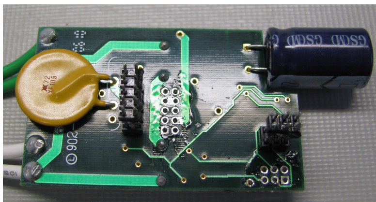
Middle PCBA, Bottom Side
