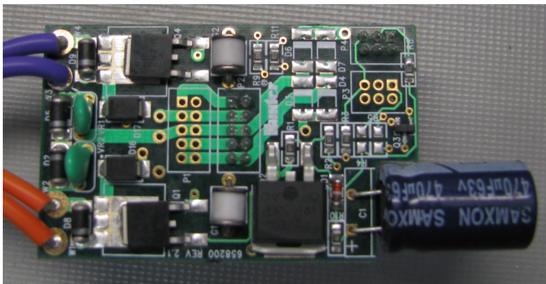
Top PCBA, Top Side
