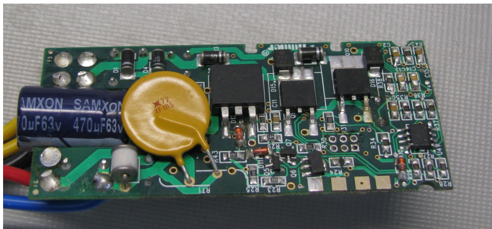
Main PCBA, Bottom Side
