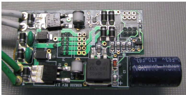
Middle PCBA, Top Side
