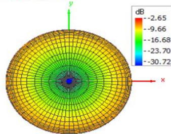
Theta = 0, Phi = 0
