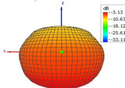
Theta = 90, Phi = 90
