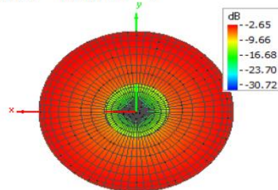
Theta = 180, Phi = 0
