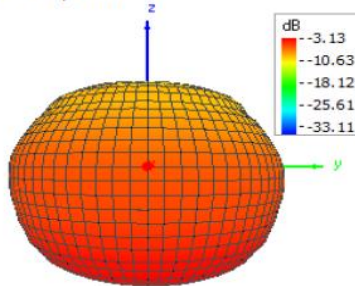
Theta = 90, Phi = 0
