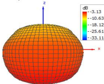
Theta = 90, Phi = 270
