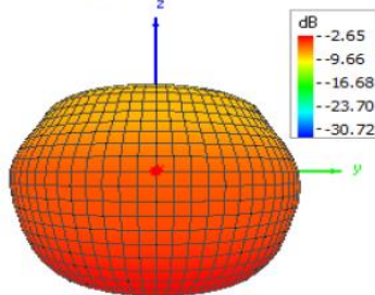
Theta = 90, Phi = 0
