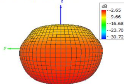
Theta = 90, Phi = 180
