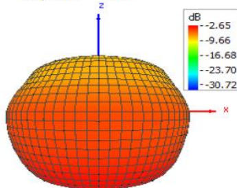
Theta = 90, Phi = 270
