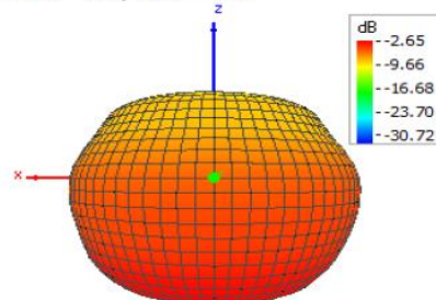
Theta = 90, Phi = 90
