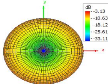
Theta = 0, Phi = 0
