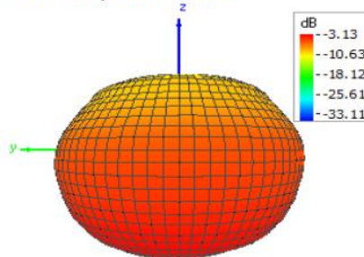
Theta = 90, Phi = 180
