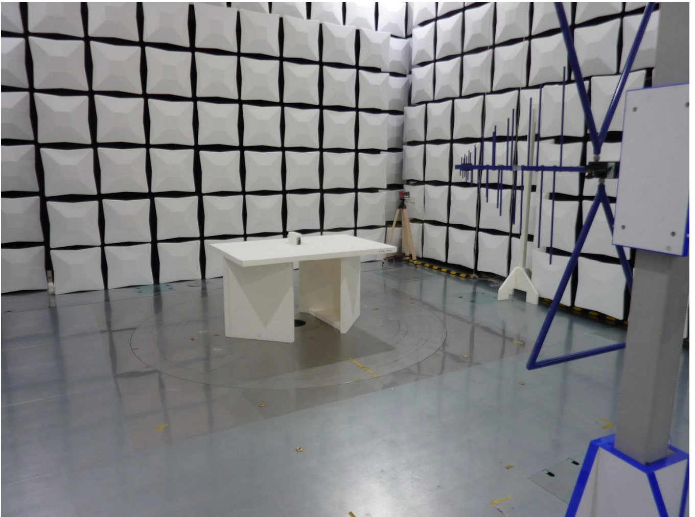
Test setup - Radiated emission 30 MHz to 1 GHz (semi anechoic chamber)
