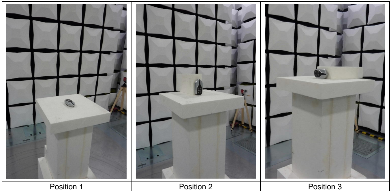
Test setup 1 GHz – 4.5 GHz - EUT (semi anechoic chamber)
