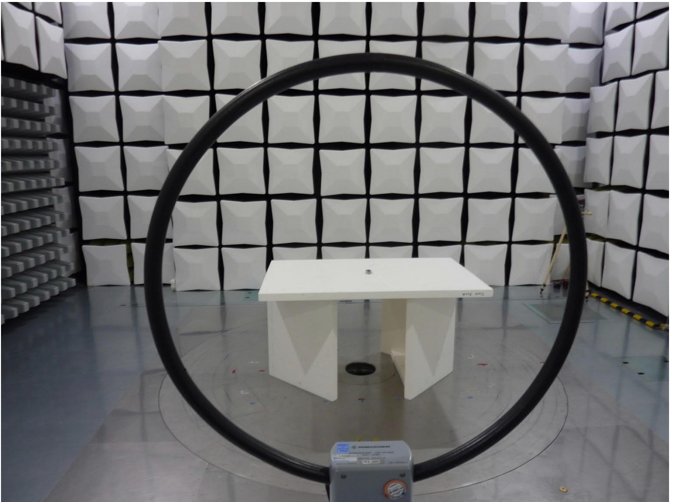
Test setup - Radiated emission 9 kHz to 30 MHz (semi anechoic chamber)
