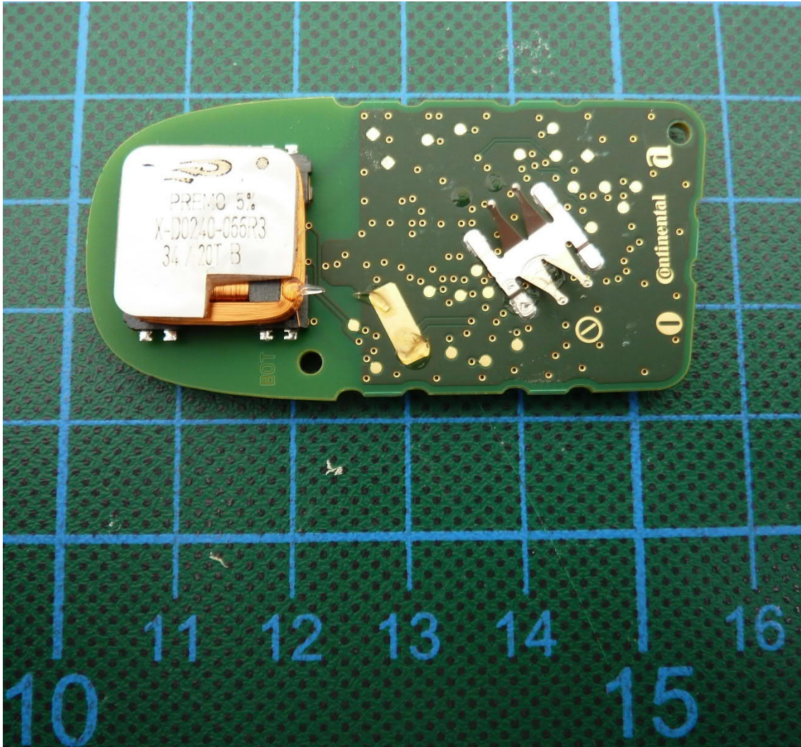
EUT – PCB bottom view
