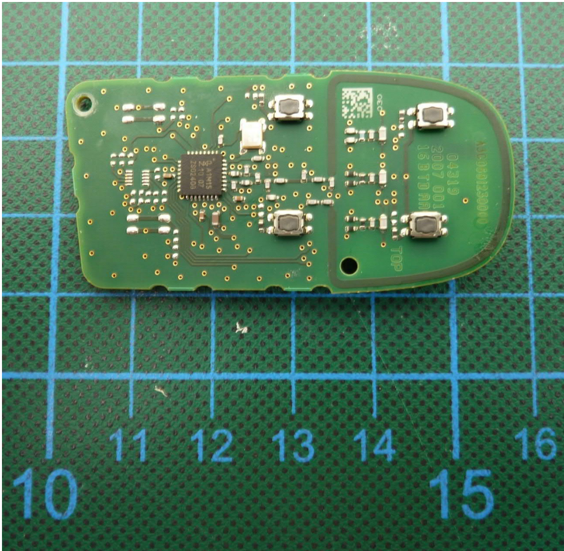
EUT – PCB top view
