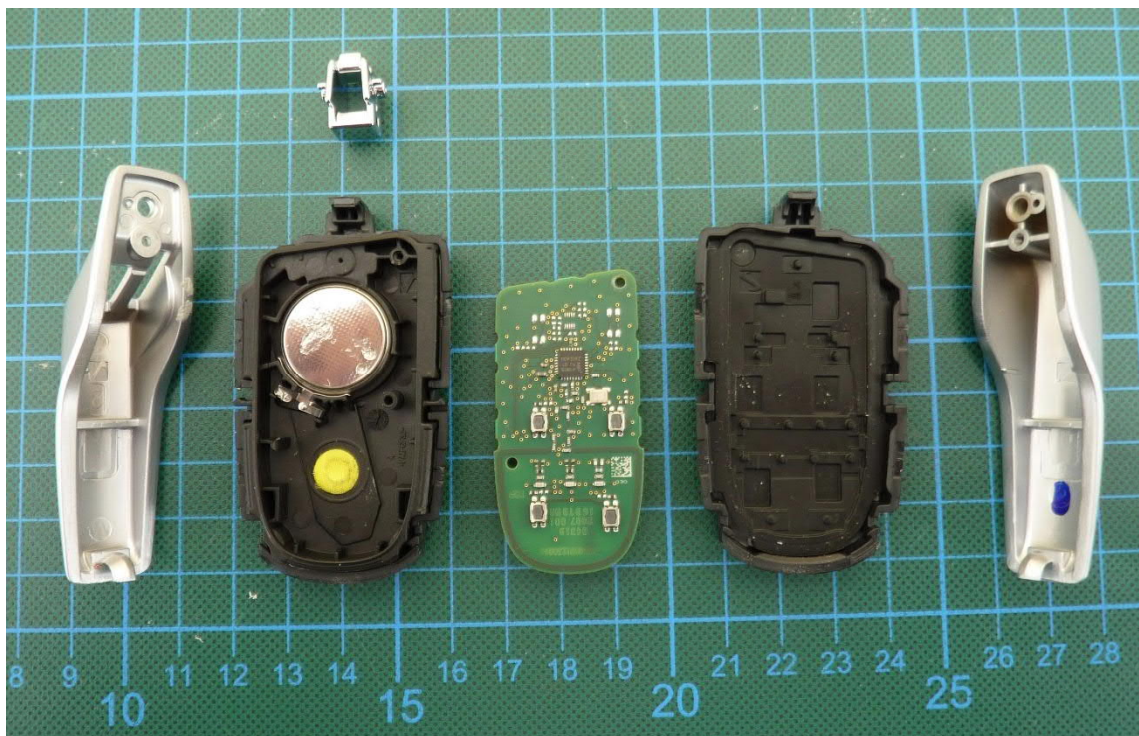
EUT – cabinet opened
