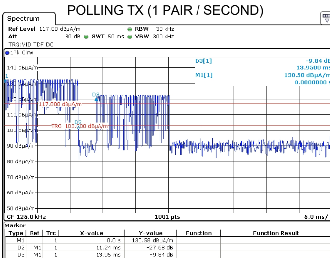
Figure 5: Pulsed Emission Characteristics (Duty Cycle).
