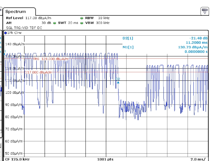
Figure 5: Pulsed Emission Characteristics (Duty Cycle).
