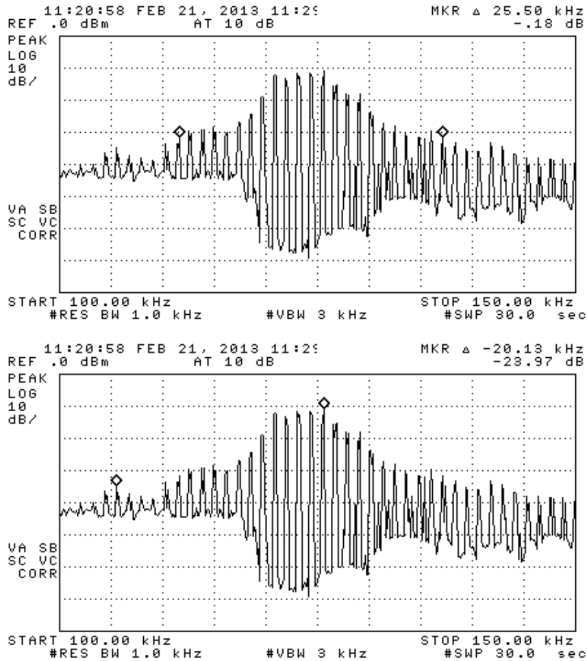
Figure 6.3(a). PEPS MODE Measured emission bandwidth of the DUT (pulsed).
