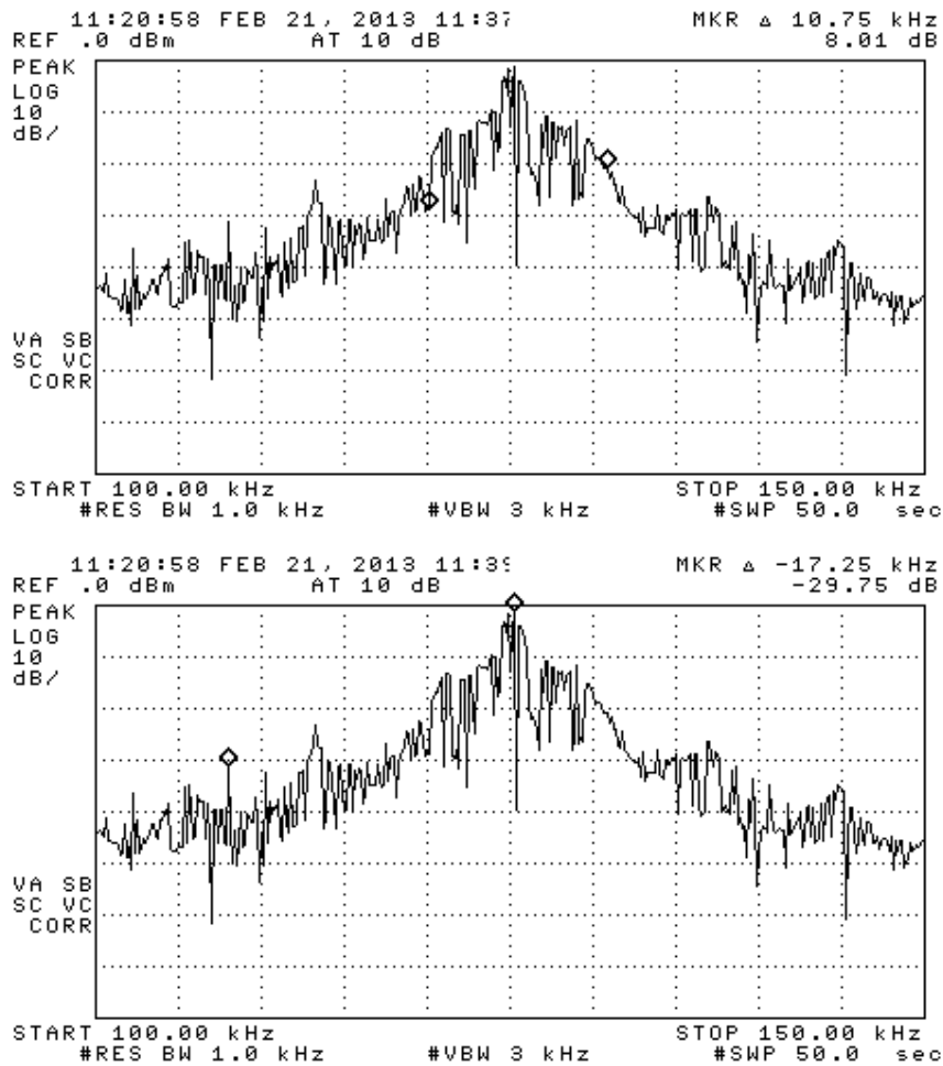
Figure 6.3(b). POLLING Measured emission bandwidth of the DUT (pulsed).
