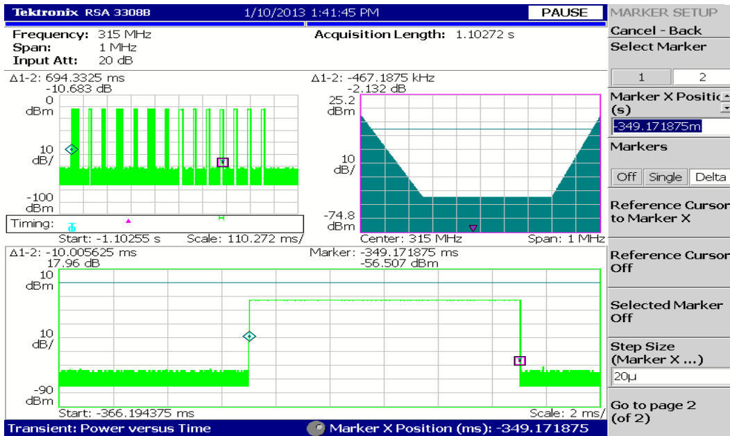
Figure 6.1(b). FSK Frames/Protocols composing worst case on time. (top) Protocol 1 (FSK), (bottom) Protocol 3 (FSK). See Description of Operation supplied with this application for details.
