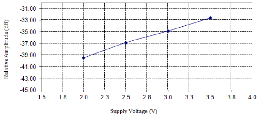
Figure 6.4. Relative emission at fundamental vs. supply voltage (pulsed).
