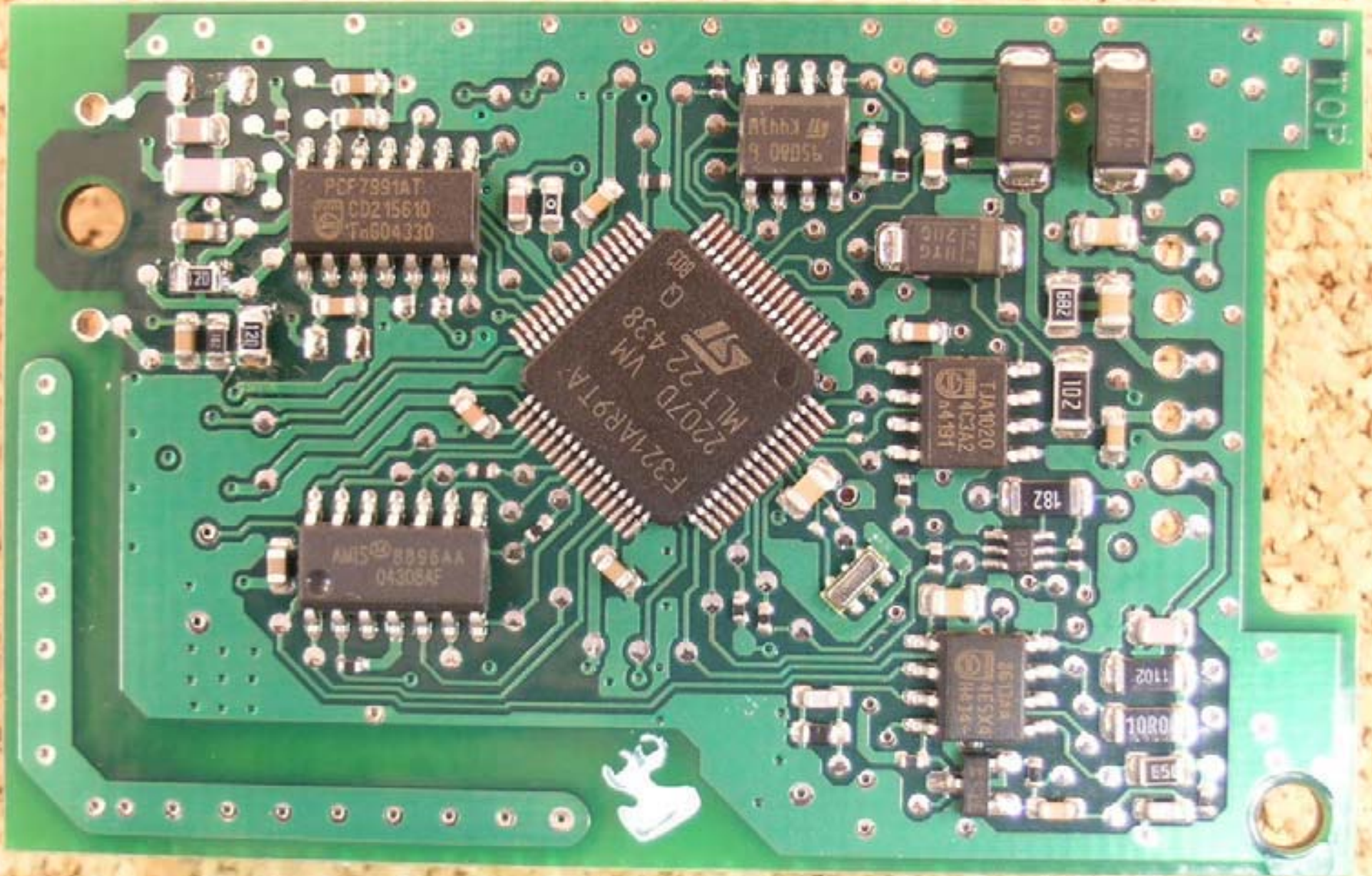
PCB (bottom)
