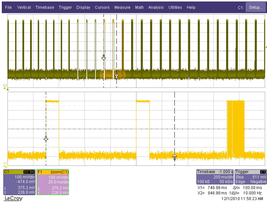
Figure 6.1(d). Worst-Case Learn-Mode modulation characteristics. (top) Worst-case transmission in 100 ms window, second FSK frame. (bottom) 100 ms window.
