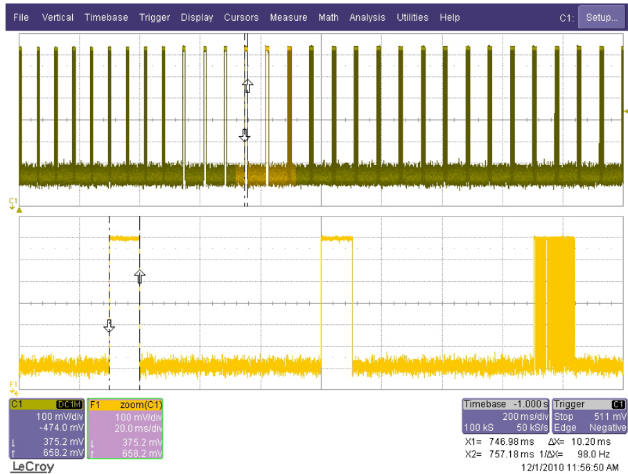
Figure 6.1(c). Worst-Case Learn-Mode modulation characteristics. (top) Manually activated transmission length, (bottom) Worst-case transmission in 100 ms window, first FSK frame.
