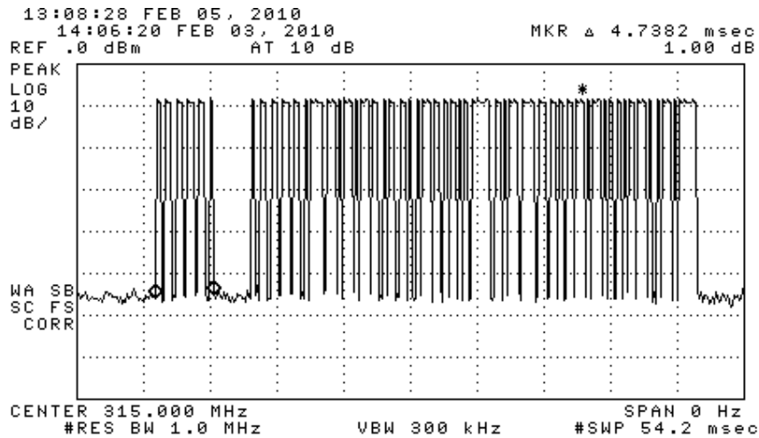
Figure 6.1(a). ASK Transmission modulation characteristics. (top) transmission after single button press, (center) expanded transmission, (bottom) expanded word.
