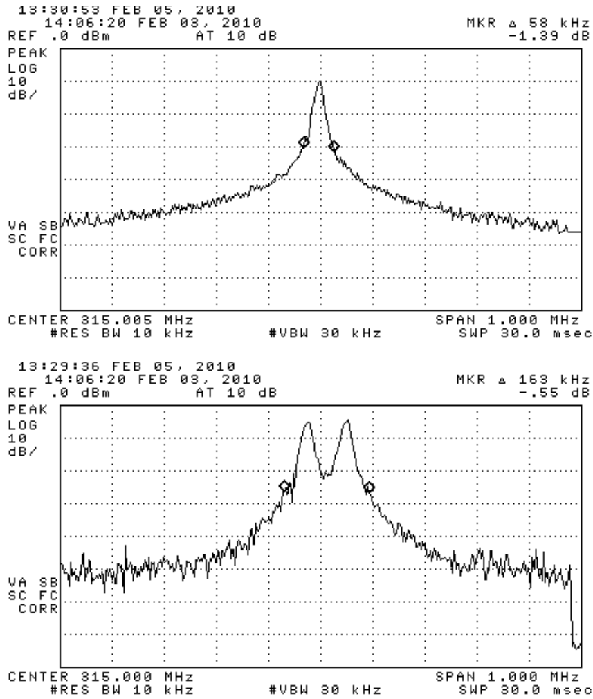
Figure 6.3. Measured emission bandwidth of the DUT (pulsed). (top) ASK, (bottom) FSK.
