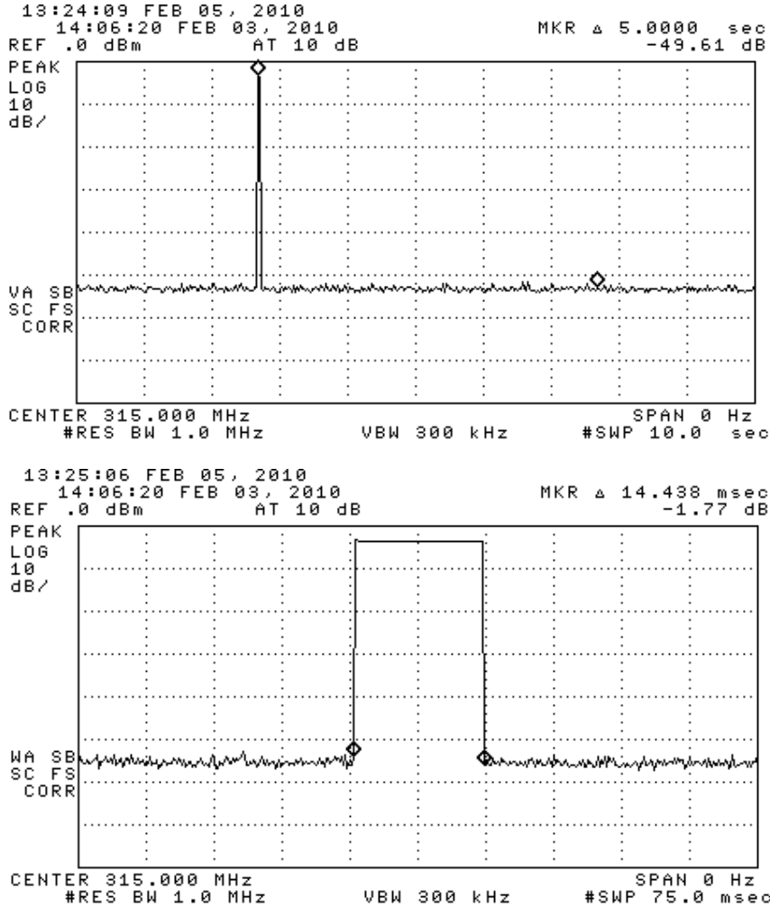
Figure 6.1(d). ASK Transmission modulation characteristics. (top) transmission after single LF interrogation, (bottom) expanded word.
