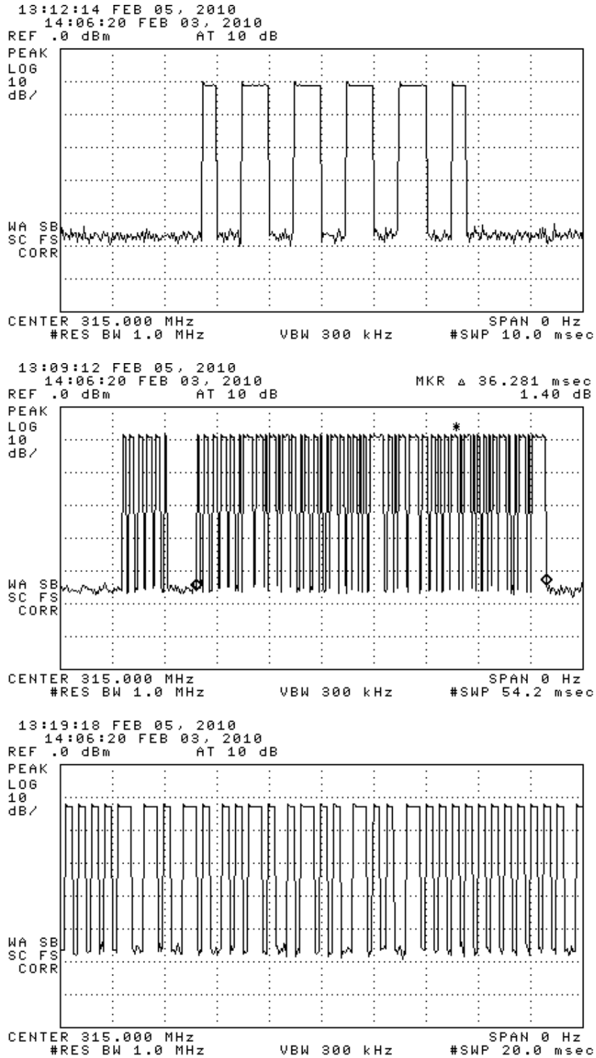
Figure 6.1(b). ASK Transmission modulation characteristics. (top) wake packet, (center) data packet, (bottom) expanded data packet showing Manchester encoding.
