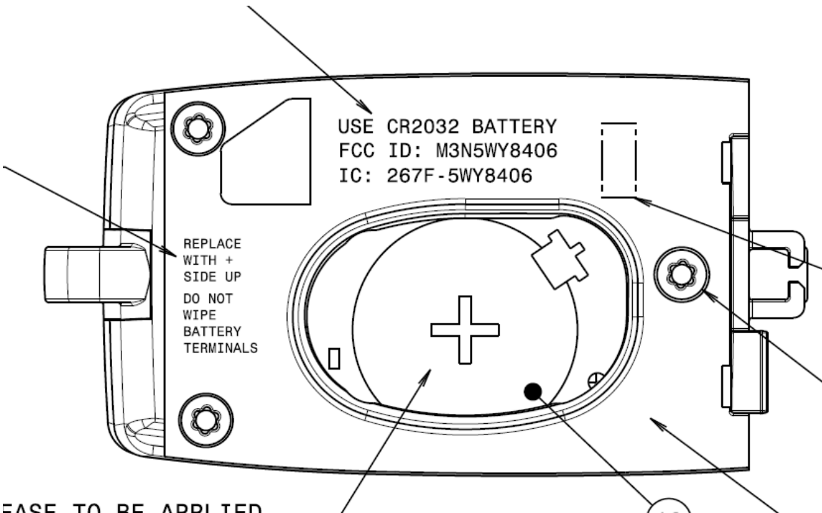
Rear View with Battery Cover Removed
