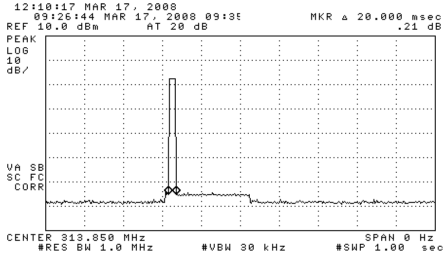
Figure 6.1(b). Transmissions modulation characteristics: (top) LF transmission, (center) expanded bit, (bottom) expanded period.
