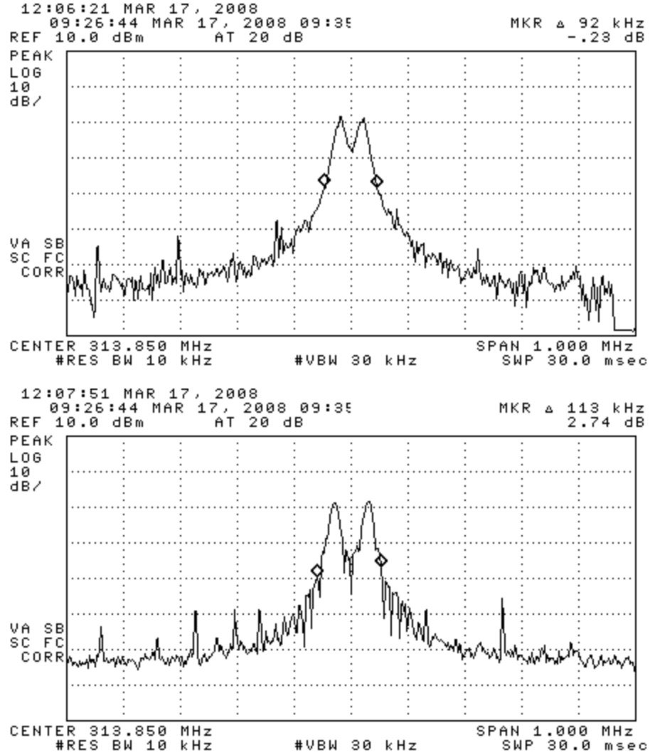
Figure 6.3. Measured bandwidth of the DUT. (top) RKE transmission, (bottom) LF activated transmission
