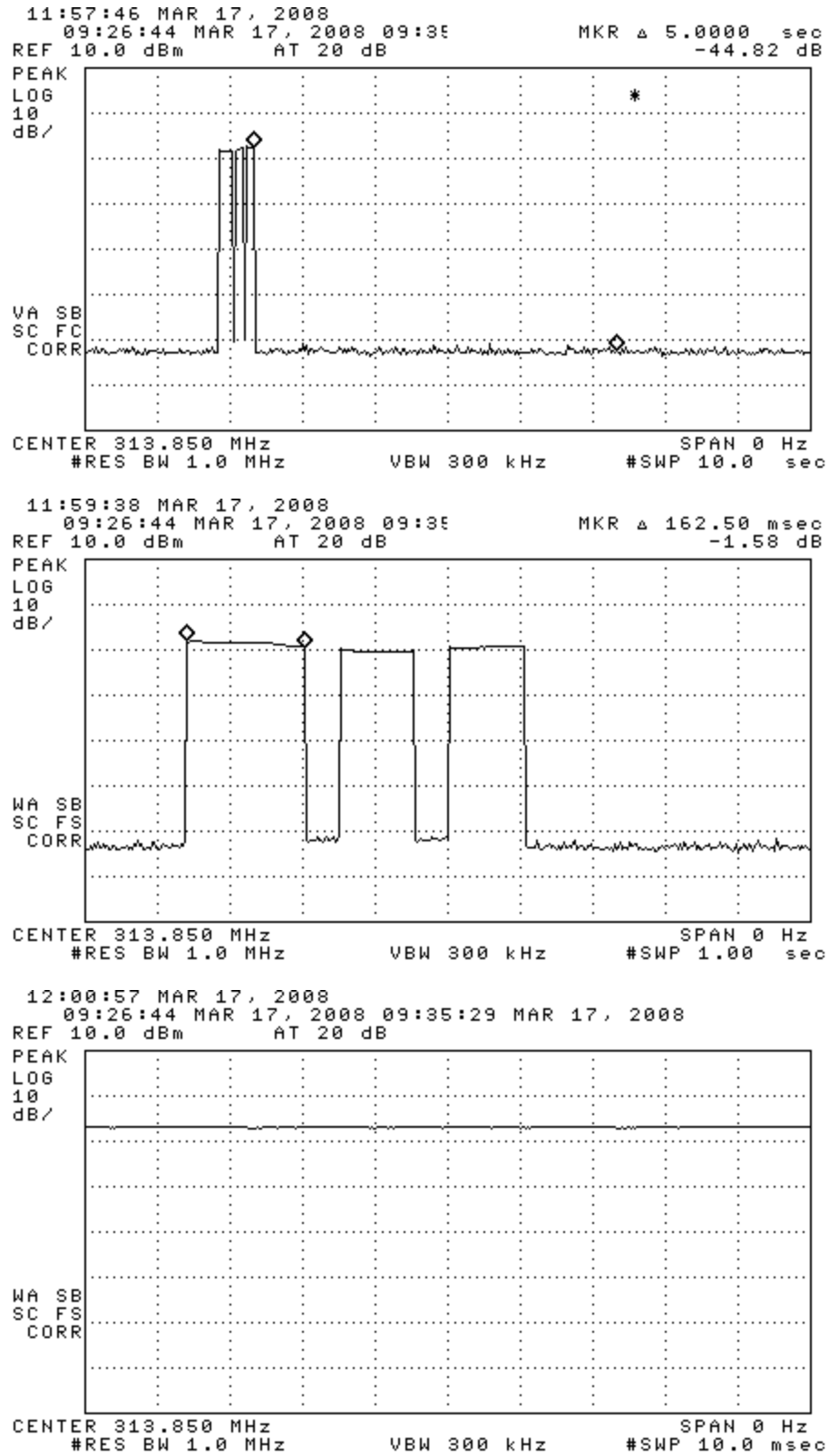
Figure 6.1(a). Transmissions modulation characteristics: (top) complete transmission, (center) expanded dataset, (bottom) duty.
