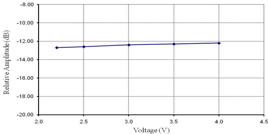
Figure 6.5. Relative emission at 315 MHz vs. supply voltage (pulsed emission).
