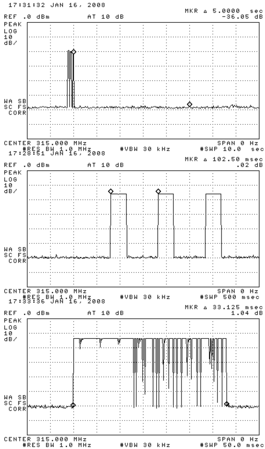
Figure 6.1(a). Transmissions modulation characteristics: (top) complete transmission, (center) 3 words, (bottom) expanded word.
