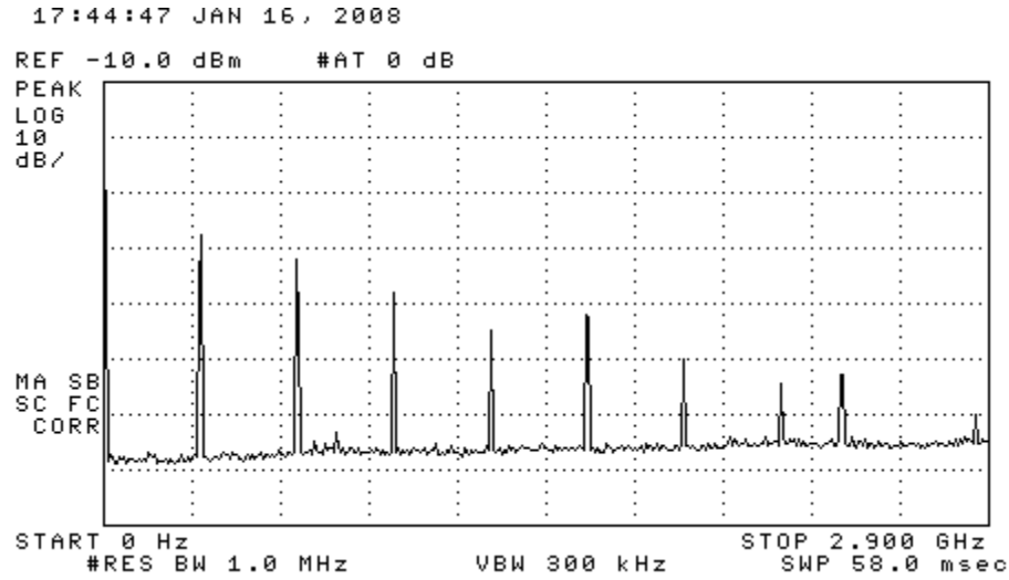
Figure 6.2. Emission spectrum of the DUT (pulsed emission). Amplitudes are indicative (not calibrated).
