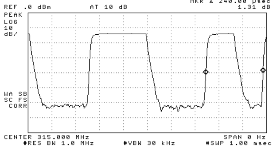
Figure 6.1(b). Transmissions modulation characteristics: (top) partial word, (center) Manchester bit, (bottom) Manchester period.
