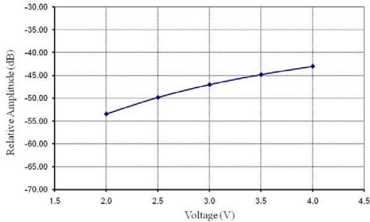
Figure 6.5. Relative emission at 315 MHz vs. supply voltage (cw emission).
