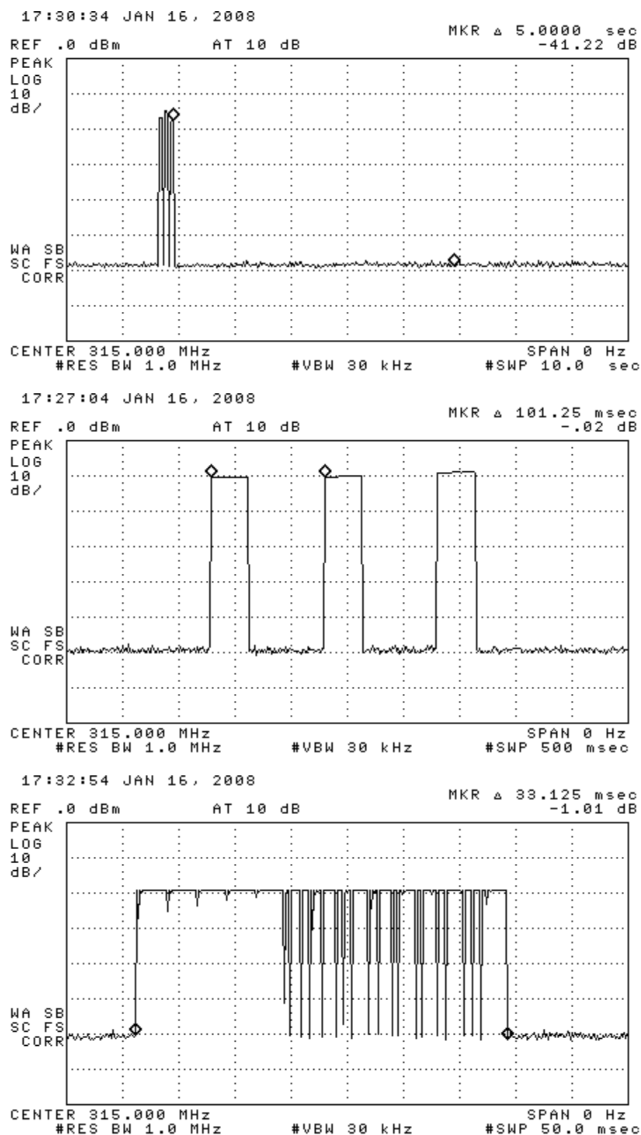
Figure 6.1(a). Transmissions modulation characteristics: (top) complete transmission, (center) expanded words, (bottom) single word.
