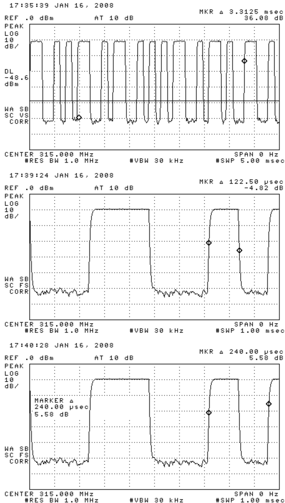
Figure 6.1(b). Transmissions modulation characteristics: (top) Manchester, (center) bit width, (bottom) bit period.
