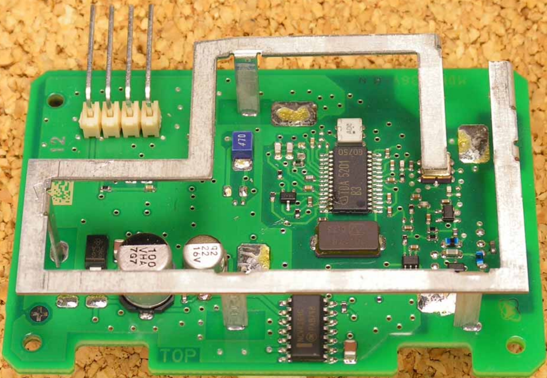
PCB (top)
