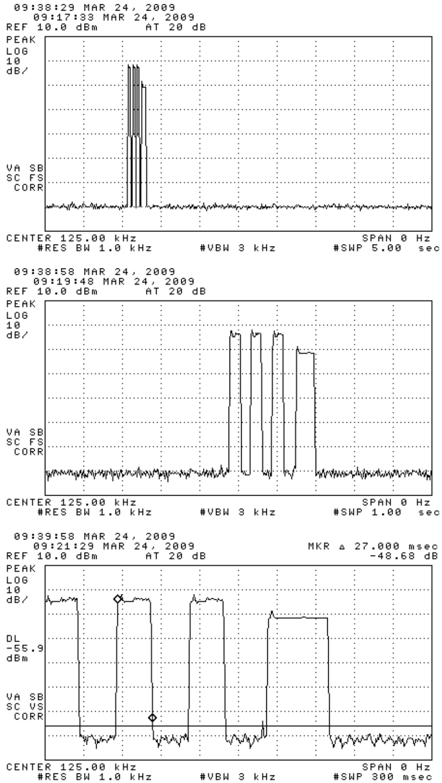
Figure 6.1(a). Transmission modulation characteristics. (top) complete transmission, (center) expanded transmission, (bottom) word length.
