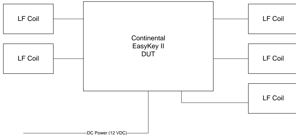
Figure 3.1 Block Diagram
