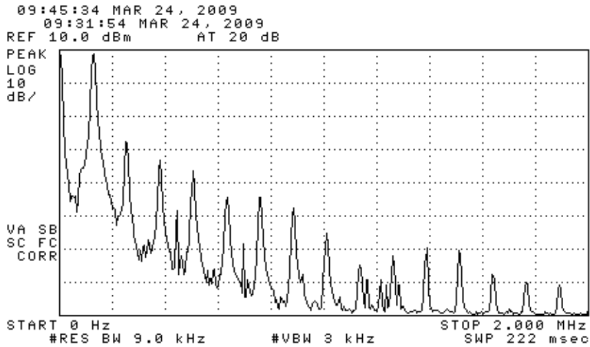
Figure 6.2. Emission spectrum of the DUT (pulsed emission).
