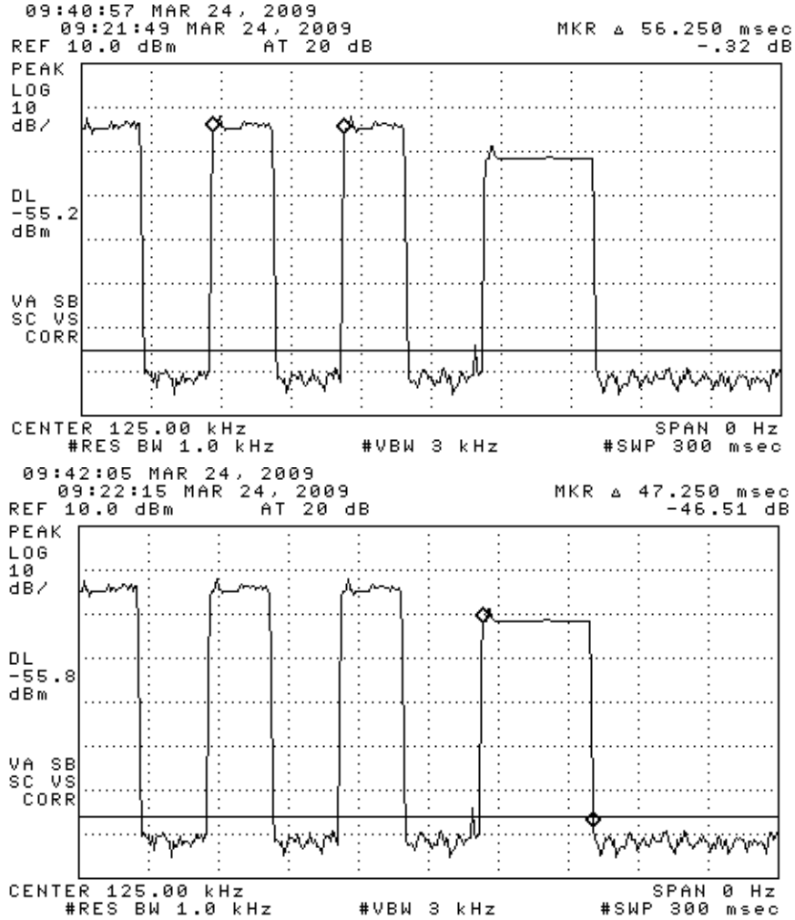
Figure 6.1(b). Transmission modulation characteristics. (top) word period, (bottom) final word
