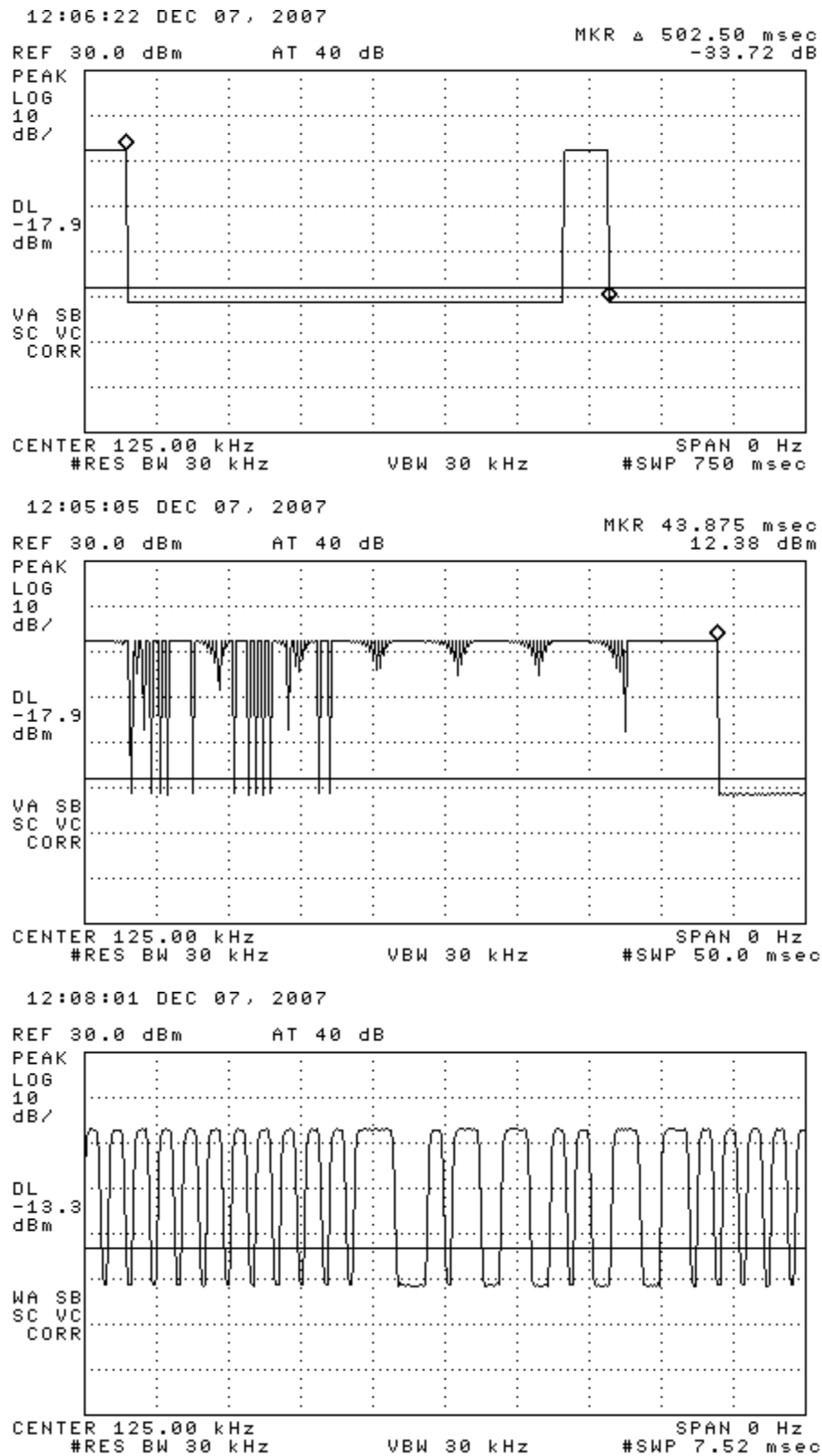
Figure 6.1(a). Transmission modulation characteristics. (top) Transmission period, (middle) Transmission length, (bottom) Manchester Encoding
