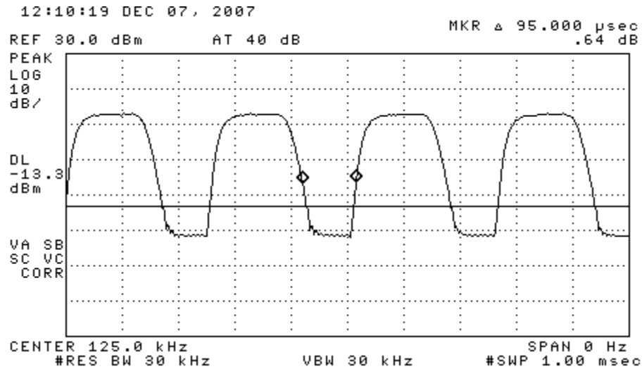
Figure 6.1(b). Manchester encoding duty cycle.
