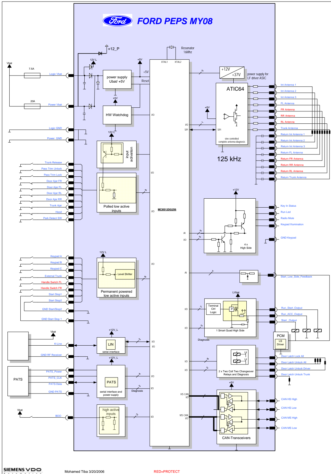
Figure 1 - PEPS System Block Diagram
