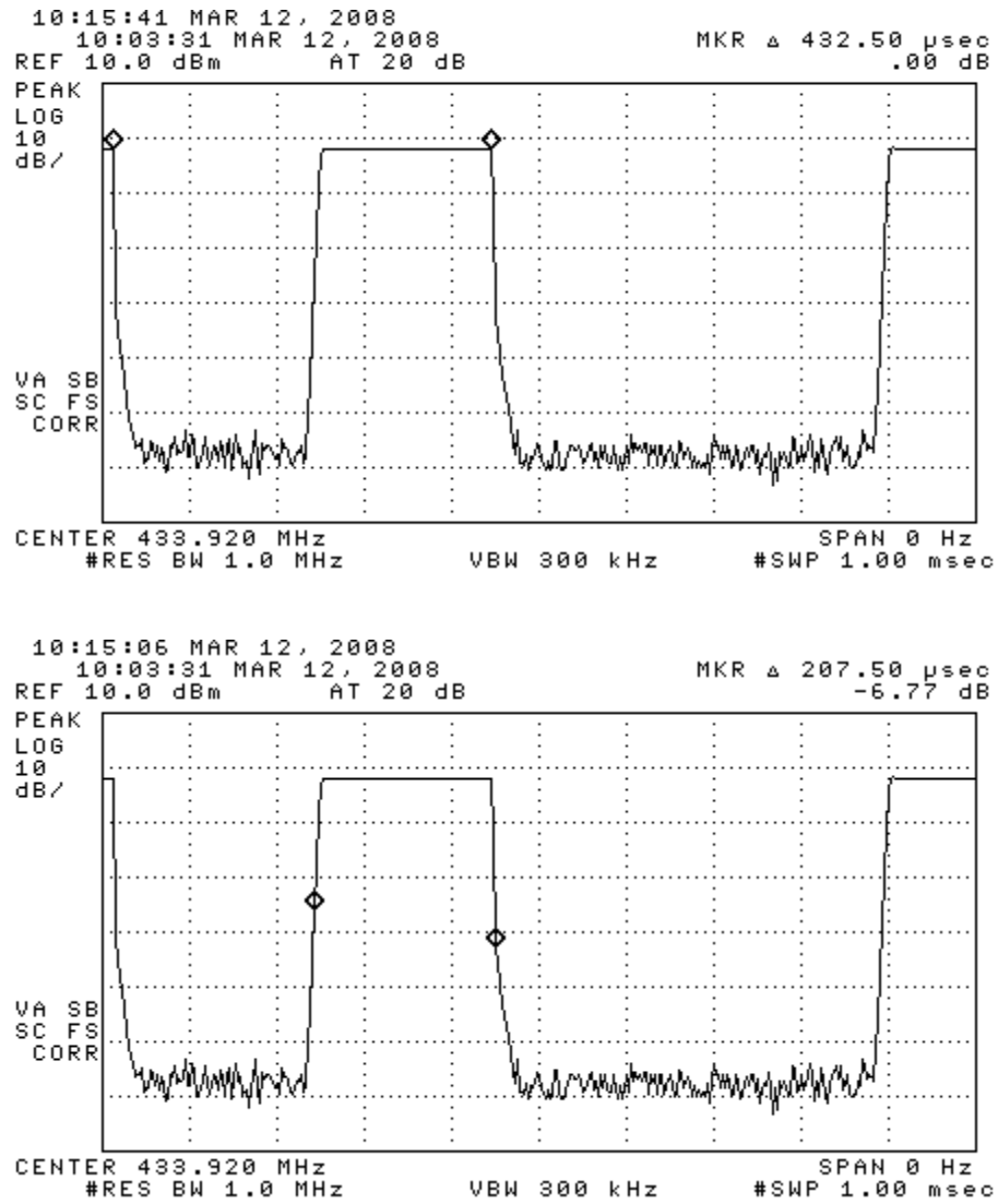
Figure 6.1(b). Transmissions modulation characteristics: (top) Manchester period, (bottom) Manchester pulse.
