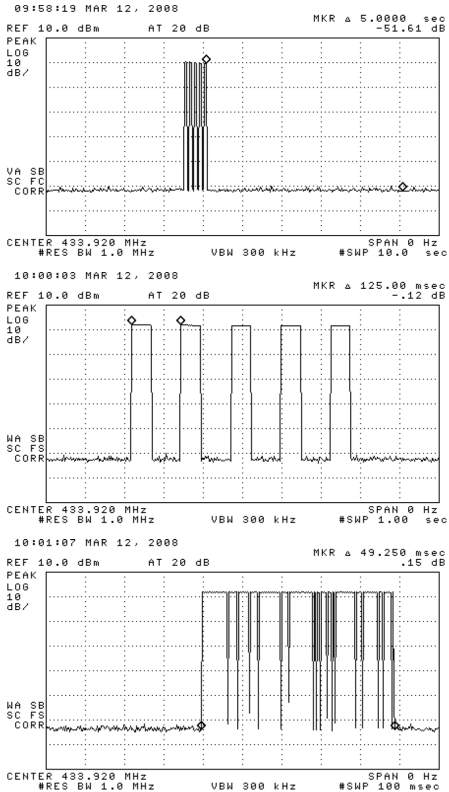
Figure 6.1(a). Transmissions modulation characteristics: (top) single transmission, (center) expanded transmission, (bottom) single word.
