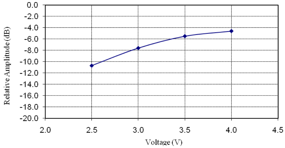
Figure 6.5. Relative emission at 315 MHz vs. supply voltage (pulsed emission).
