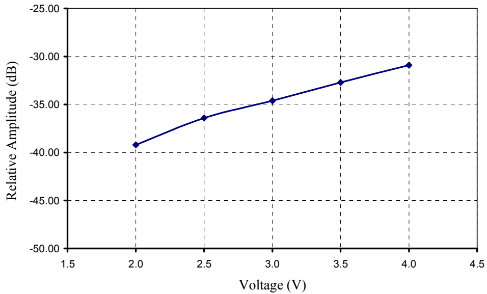
Figure 6.5. Relative emission at 433.9 MHz vs. supply voltage (pulsed emission).
