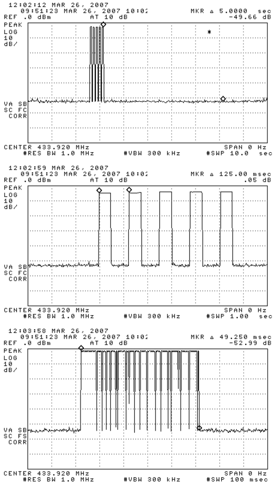
Figure 6.1(a). Transmissions modulation characteristics: (top) complete transmission, (center) expanded bit, (bottom) expanded period.
