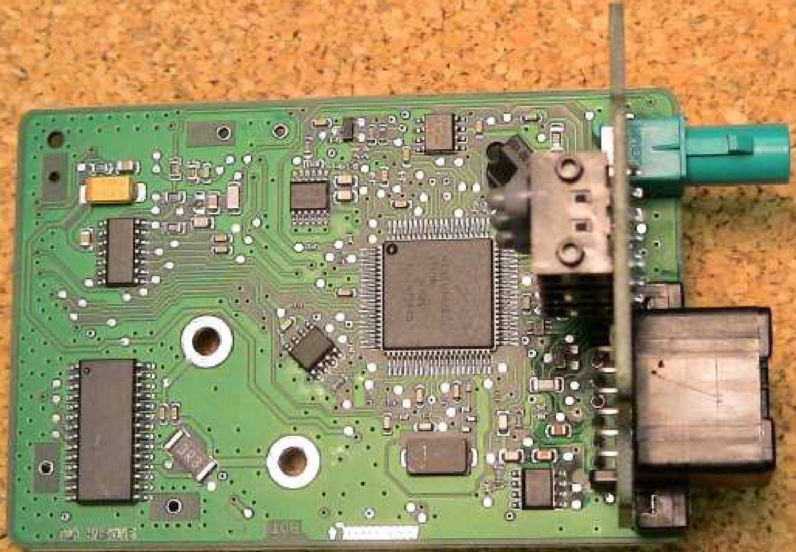
PCB (top)
