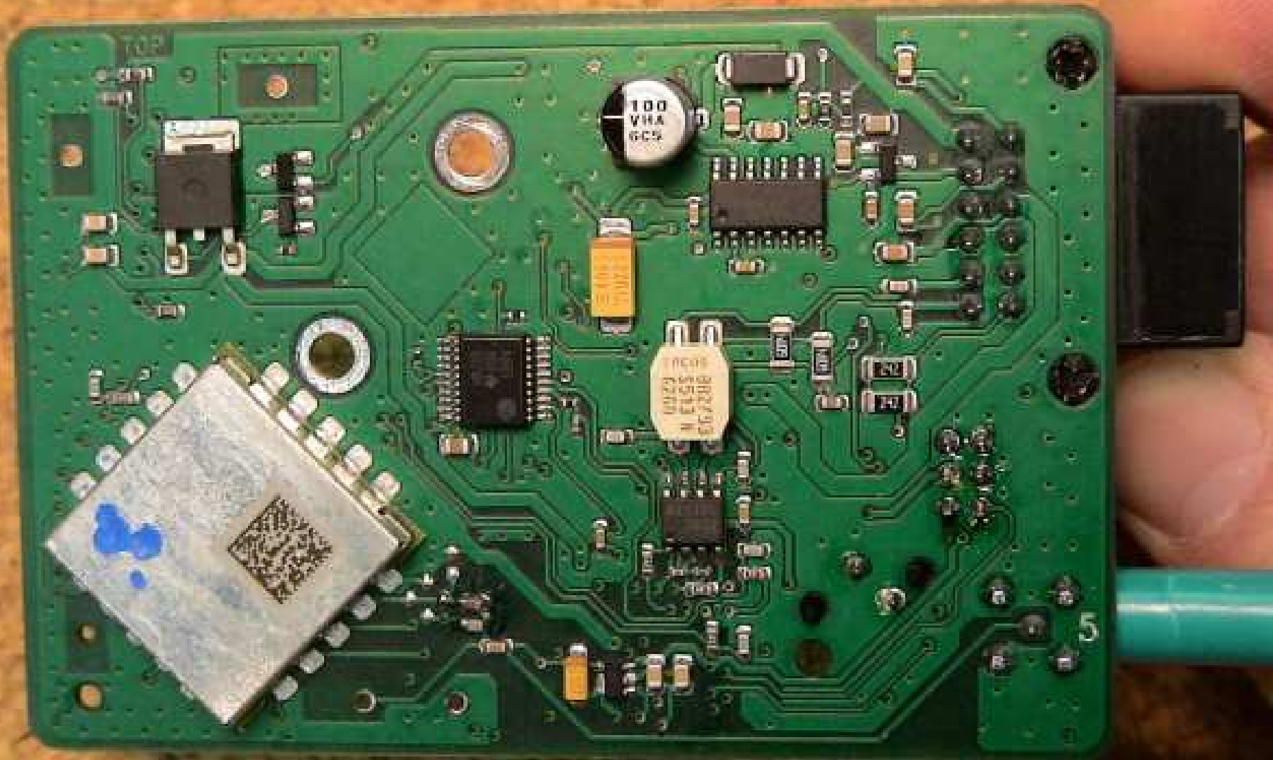
PCB (bottom)
