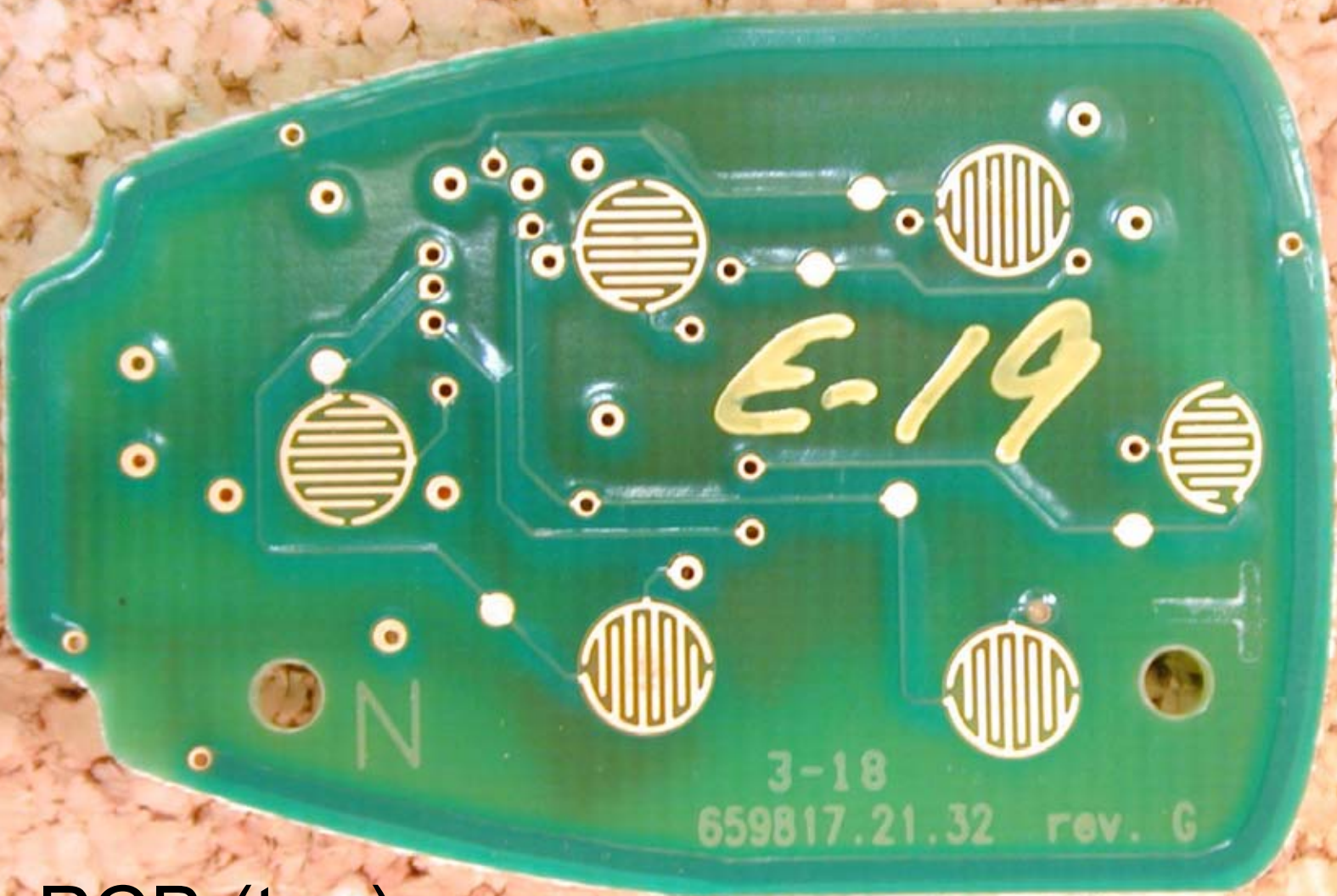
PCB (top)
