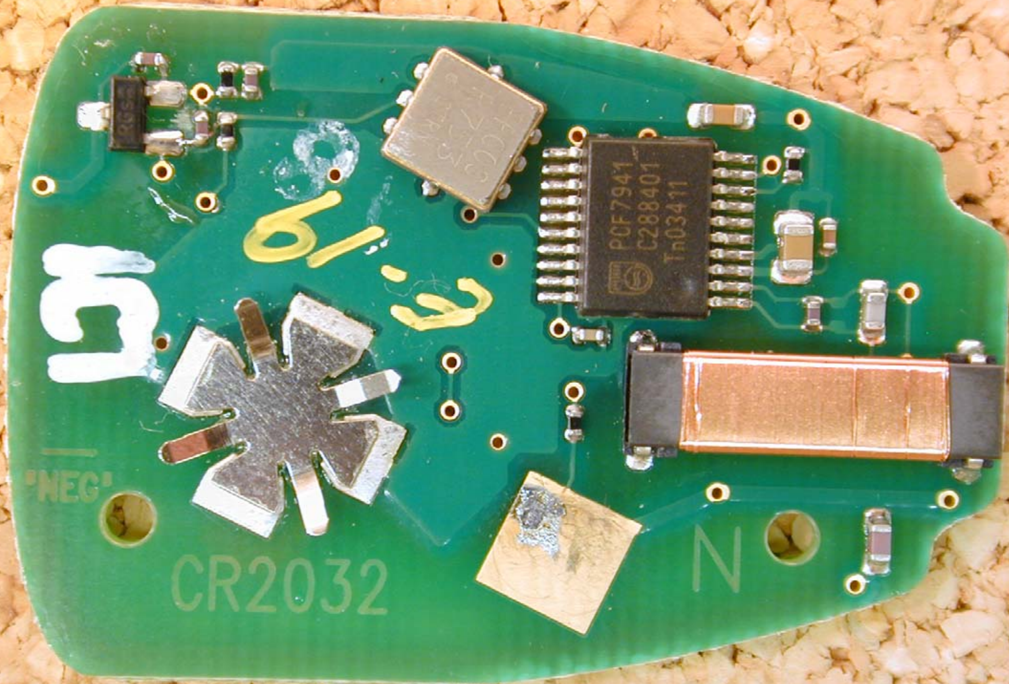
PCB (bottom)
