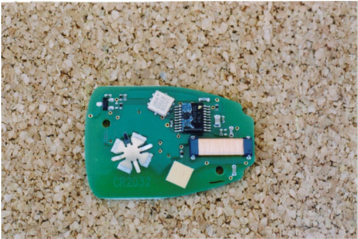
5WY72XX Transmitter – PCB Bottom
