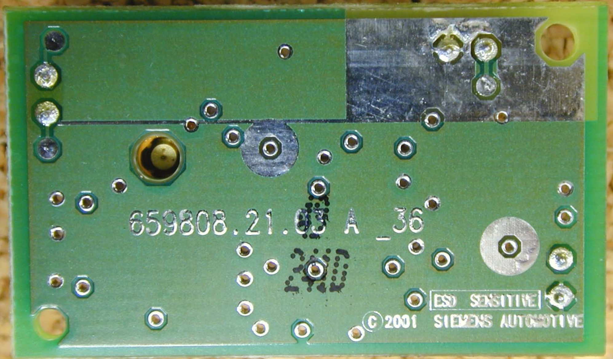
Daughterboard Bottom
