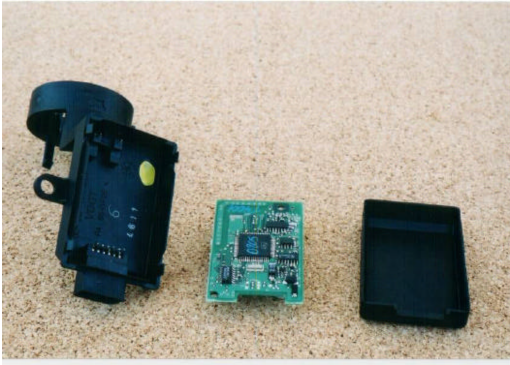
5WY7078 Immobilizer– Case Open Top
