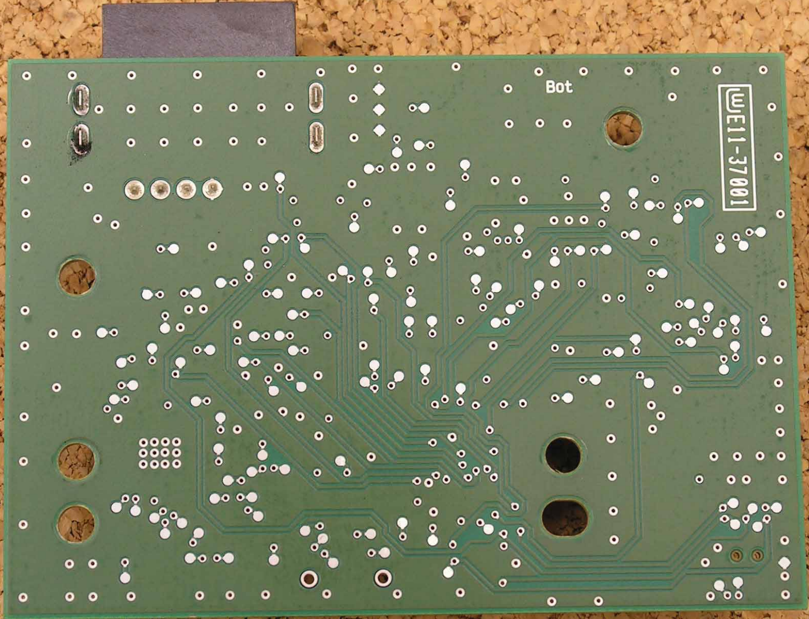
PCB (bottom)
