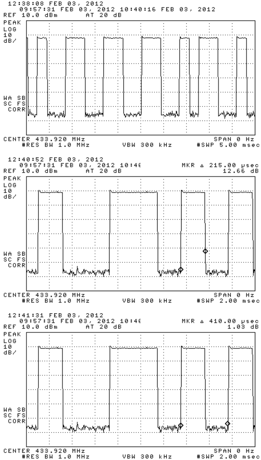
Figure 6.1(c). Data Word characteristics. (top) encoding, (center) pulse length, (bottom) pulse period.
