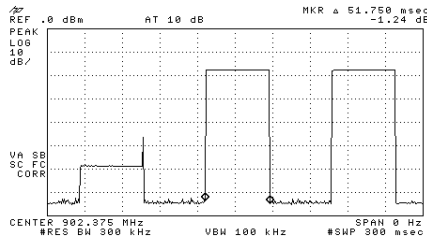
Figure 5: Fundamental Emission Pulsed Operation.
