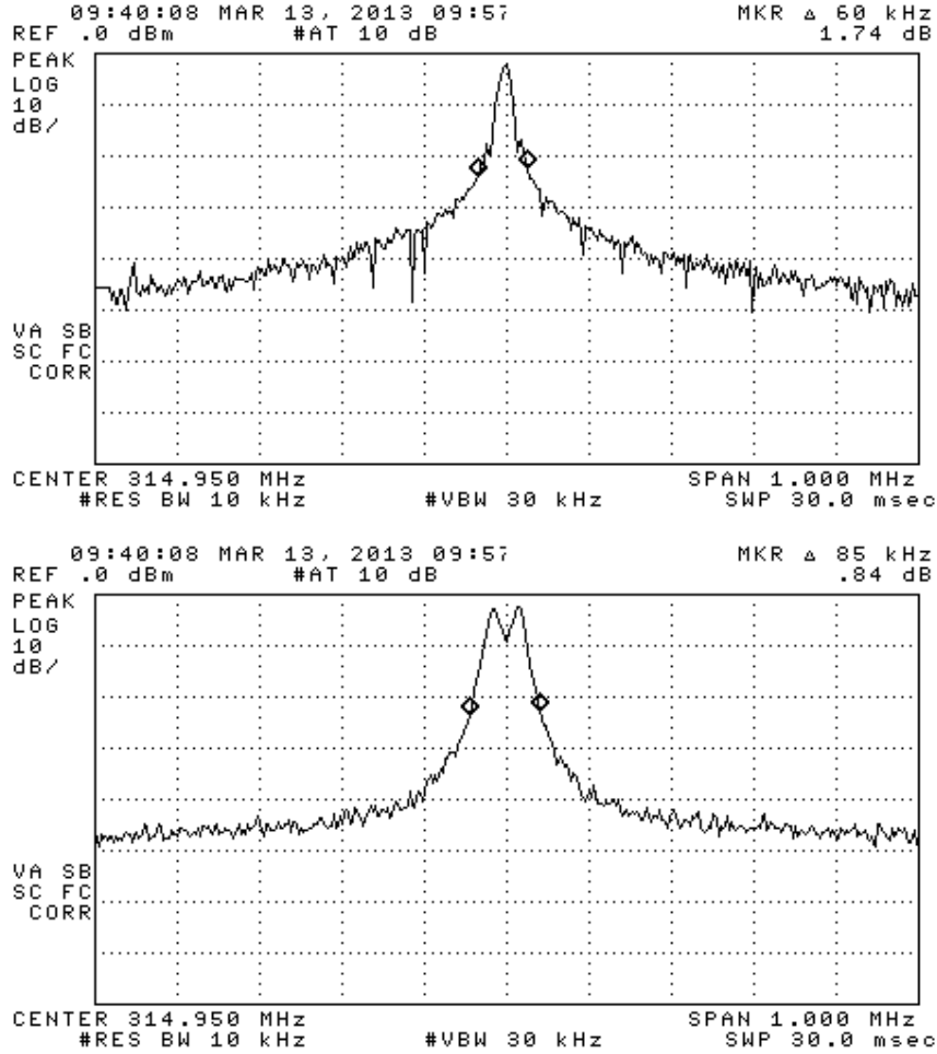
Figure 6.3. Measured emission bandwidth of the DUT (pulsed).
