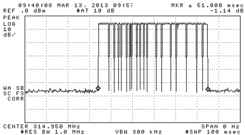
Figure 6.1. Manually Activated ASK Transmission Characteristics. (top) single transmission, (center) frame period, (bottom) frame length.
