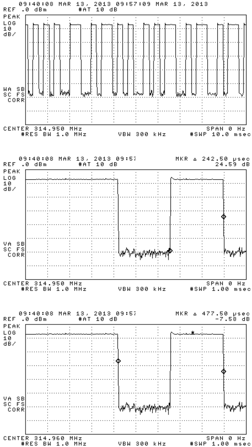
Figure 6.1(b). ASK Transmission Characteristics. (top) ASK Manchester encoding, (center) ASK bit width, (bottom) ASK bit period.
