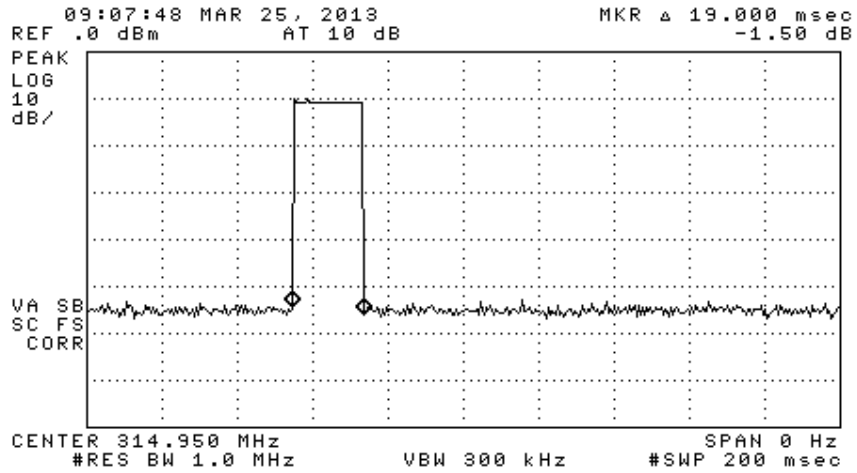
Figure 6.1(c). Manually Activated LF Triggered FSK Transmission. (top) complete transmission, (bottom) FSK Frame length.
