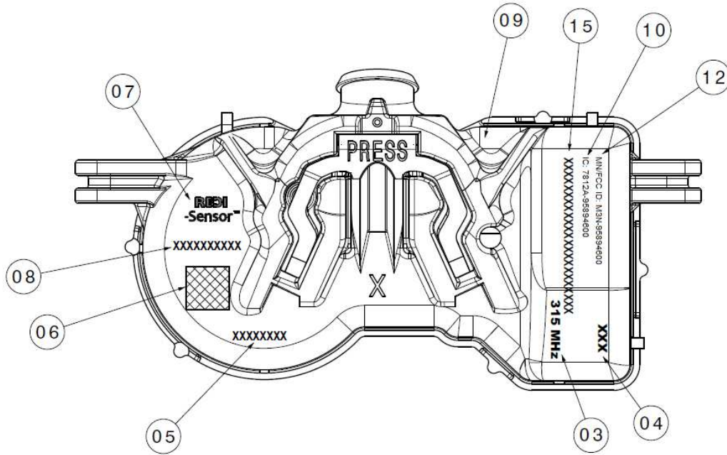
LASER MARKING - HOUSING SIDE (TOP VIEW) Scale: 3:1
