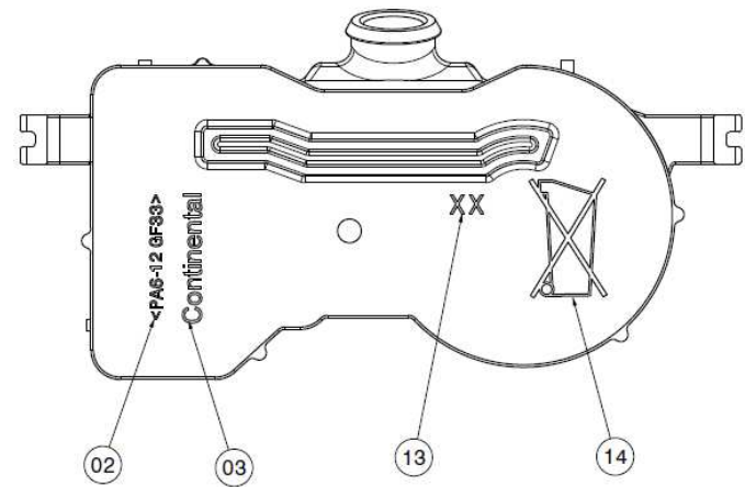
LASER MARKING - COVER SIDE (BOTTOM VIEW) Scale: 3:1
