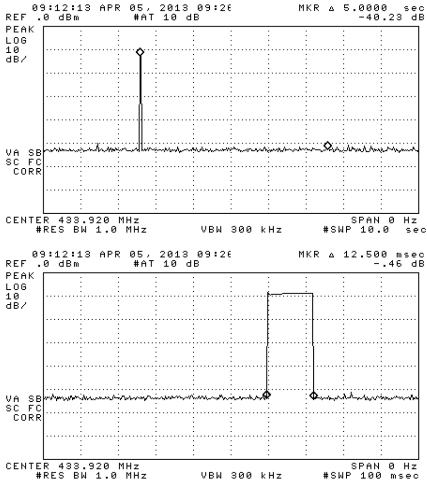
Figure 6.1(c). FSK Transmission modulation characteristics. (top) complete transmission, (bottom) expanded frame.
