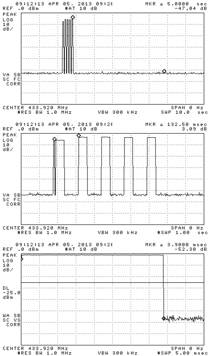
Figure 6.1(a). ASK Transmission modulation characteristics. (top) complete transmission, (center) expanded transmission, (bottom) initial “wake” pulse.
