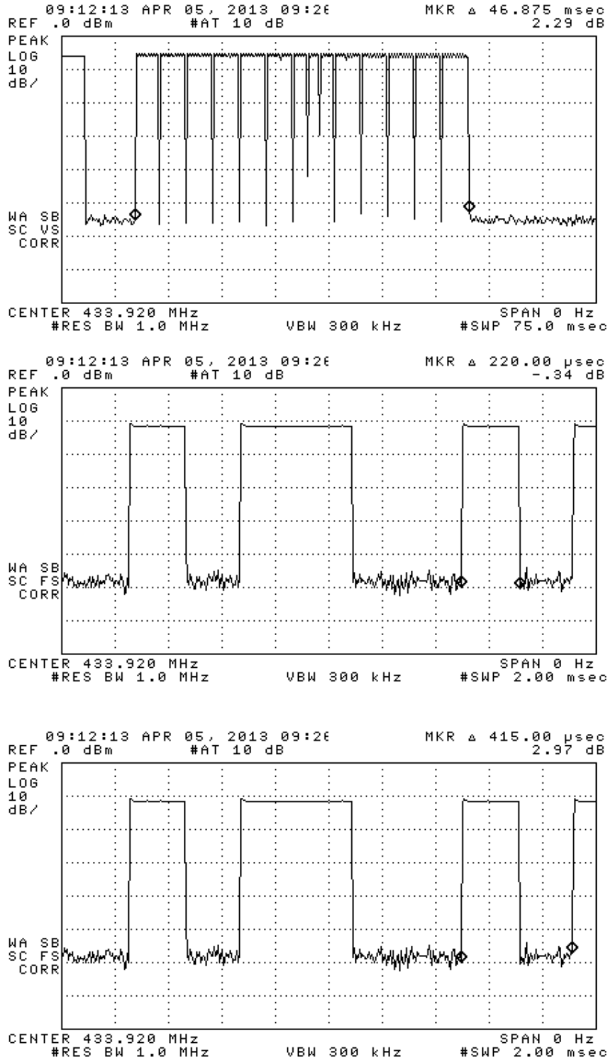
Figure 6.1(b). ASK Transmission modulation characteristics. (top) Manchester frame, (center) Manchester pulse width, (bottom) Manchester period.
