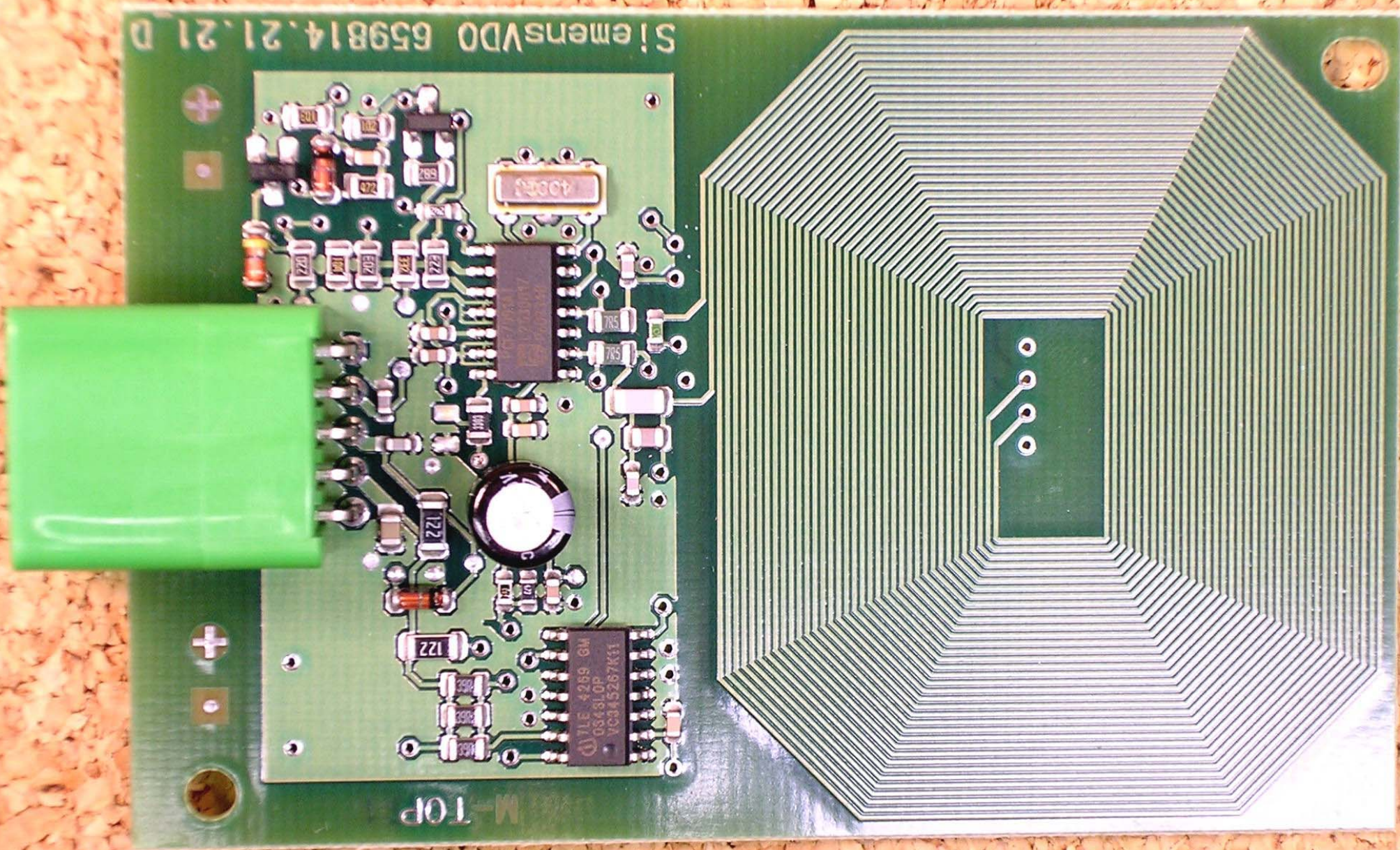
PCB (top)
