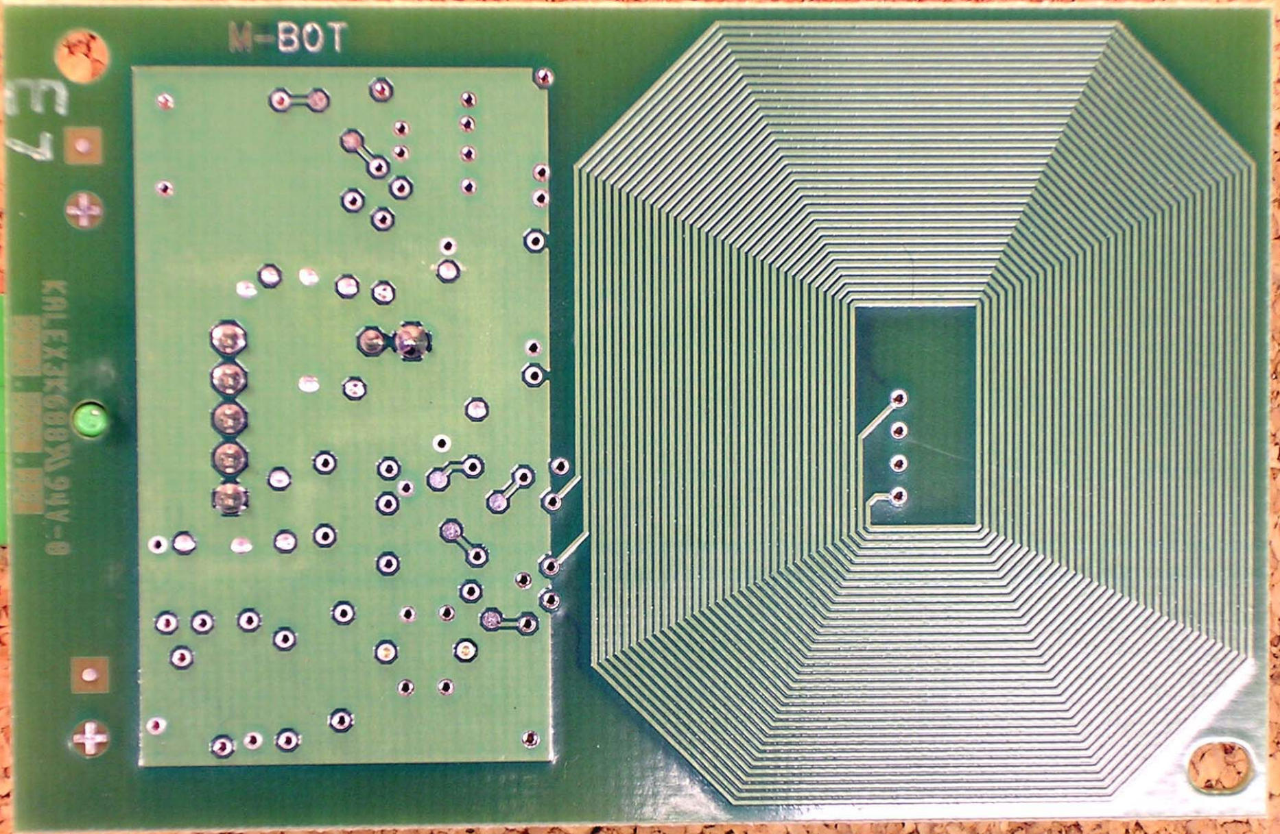
PCB (bottom)
