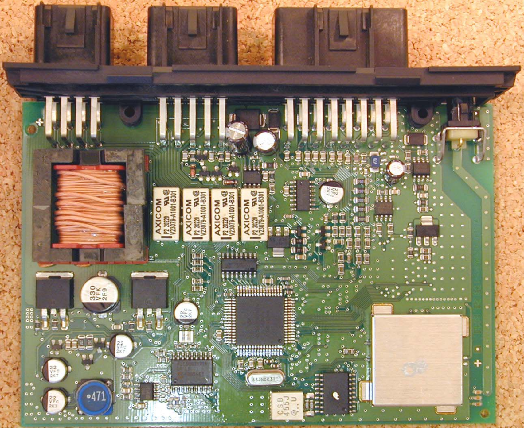
PCB (top)
