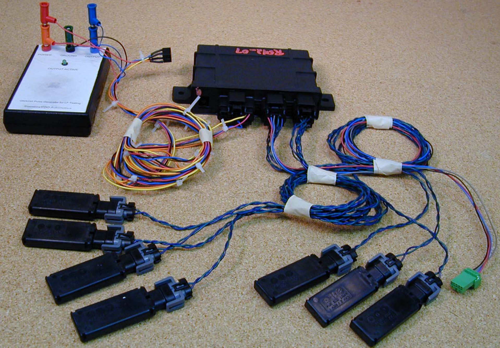
DUT with harness, test box, and activator coils
