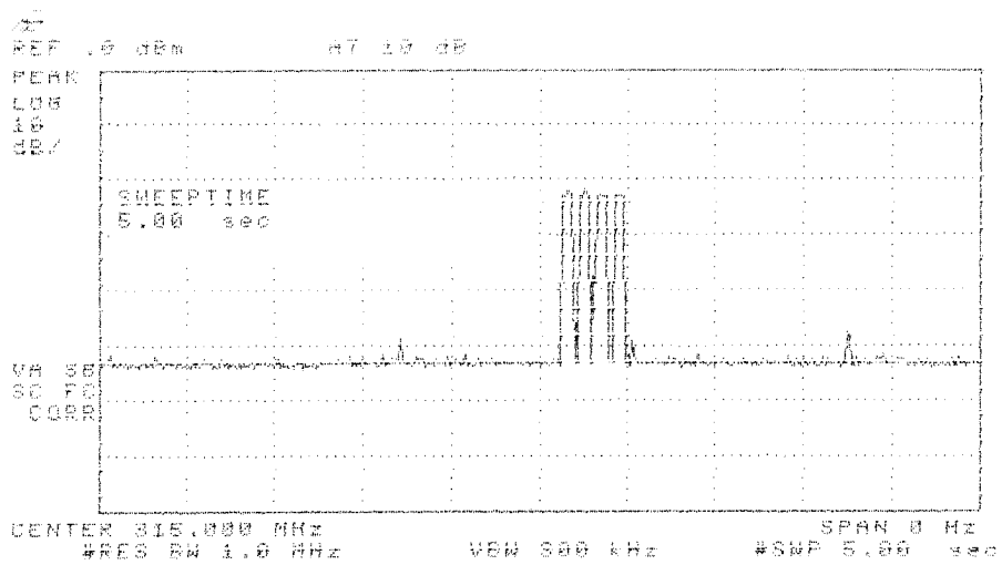
Figure 6.5. Emission for instant activation.
