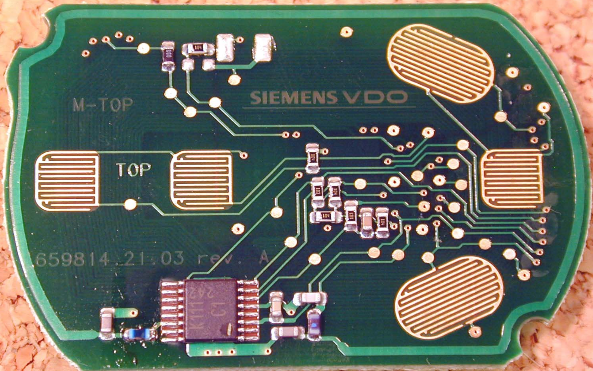
PCB (top)
