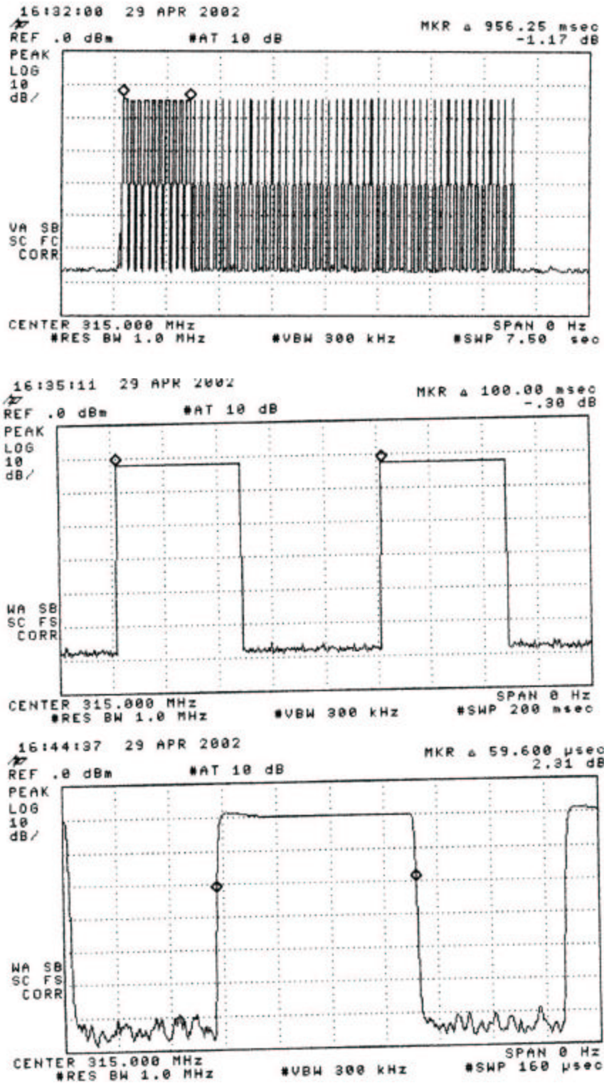
Figure 6.1. Transmitter modulation characteristics: (top) complete transmission, (center) expanded bit, (bottom) expanded period.
