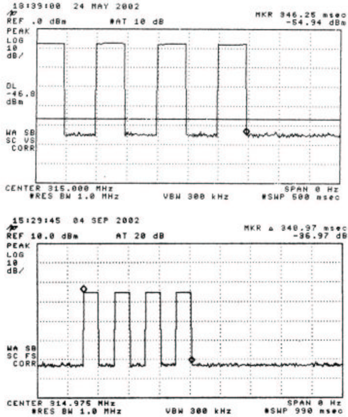
Figure 6.4. Transmitter 5 sec. transmission limit verification. Top (remote activation), bottom (manual activation).
