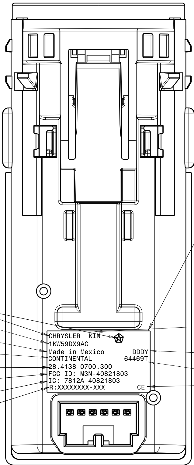
Label area for laser printing Connector side view (Text Ht 1.00 mm)
