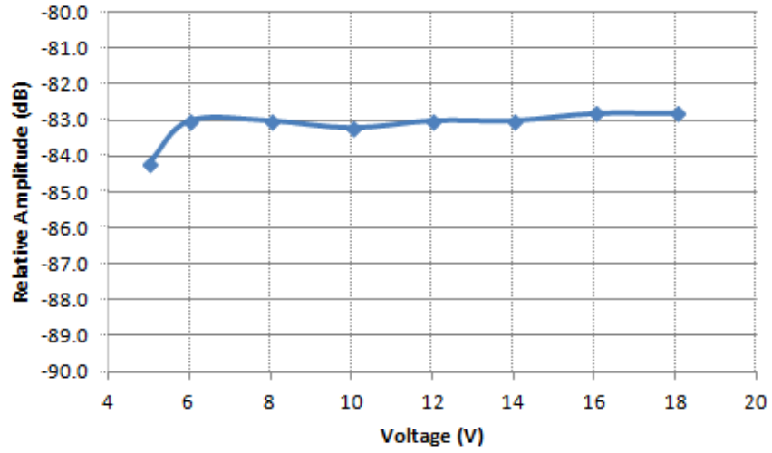
Figure 6.4. Relative emission vs. supply voltage.
