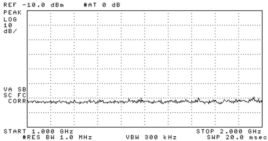
Figure 6.2. Emissions measured at 3 meters in chamber, 1000-2000 MHz. (emission at marker is background)
