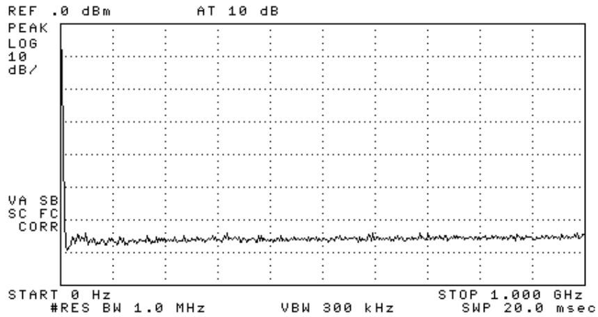
Figure 6.1. Emissions measured at 3 meters in chamber, 0-1000 MHz.
