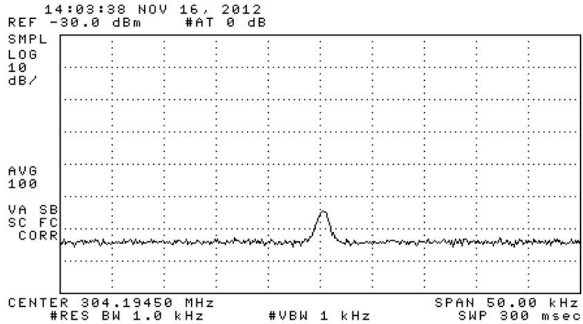
Figure 6.3. Relative receiver emission(s).
