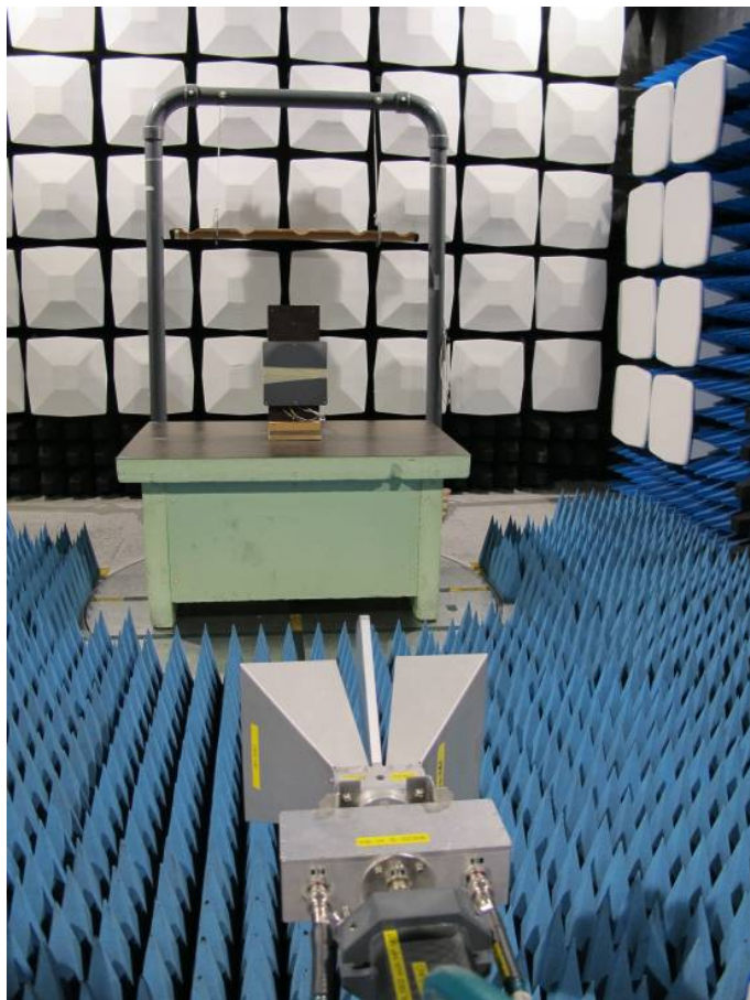
Radiated emission above 1 GHz
